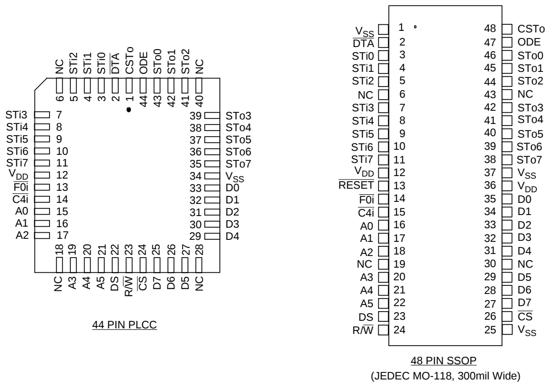
Figure 2 - Pin Connections
