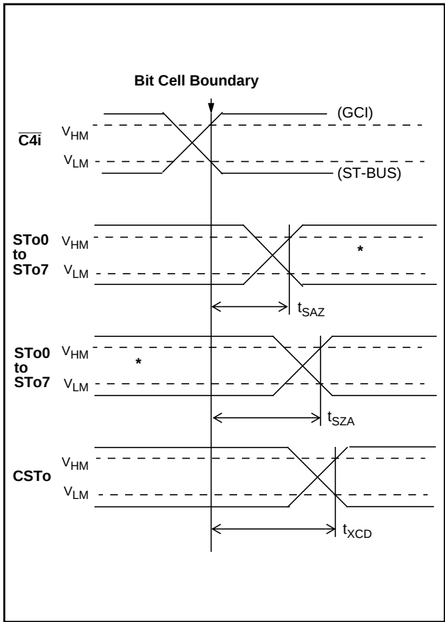
Figure 14 - Serial Outputs and External Control
