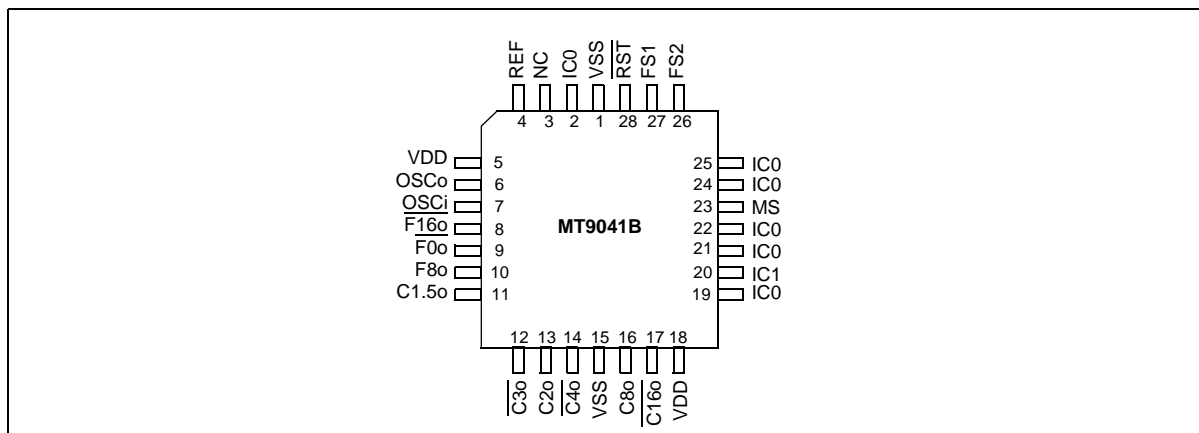
Figure 2 - Pin Connections
