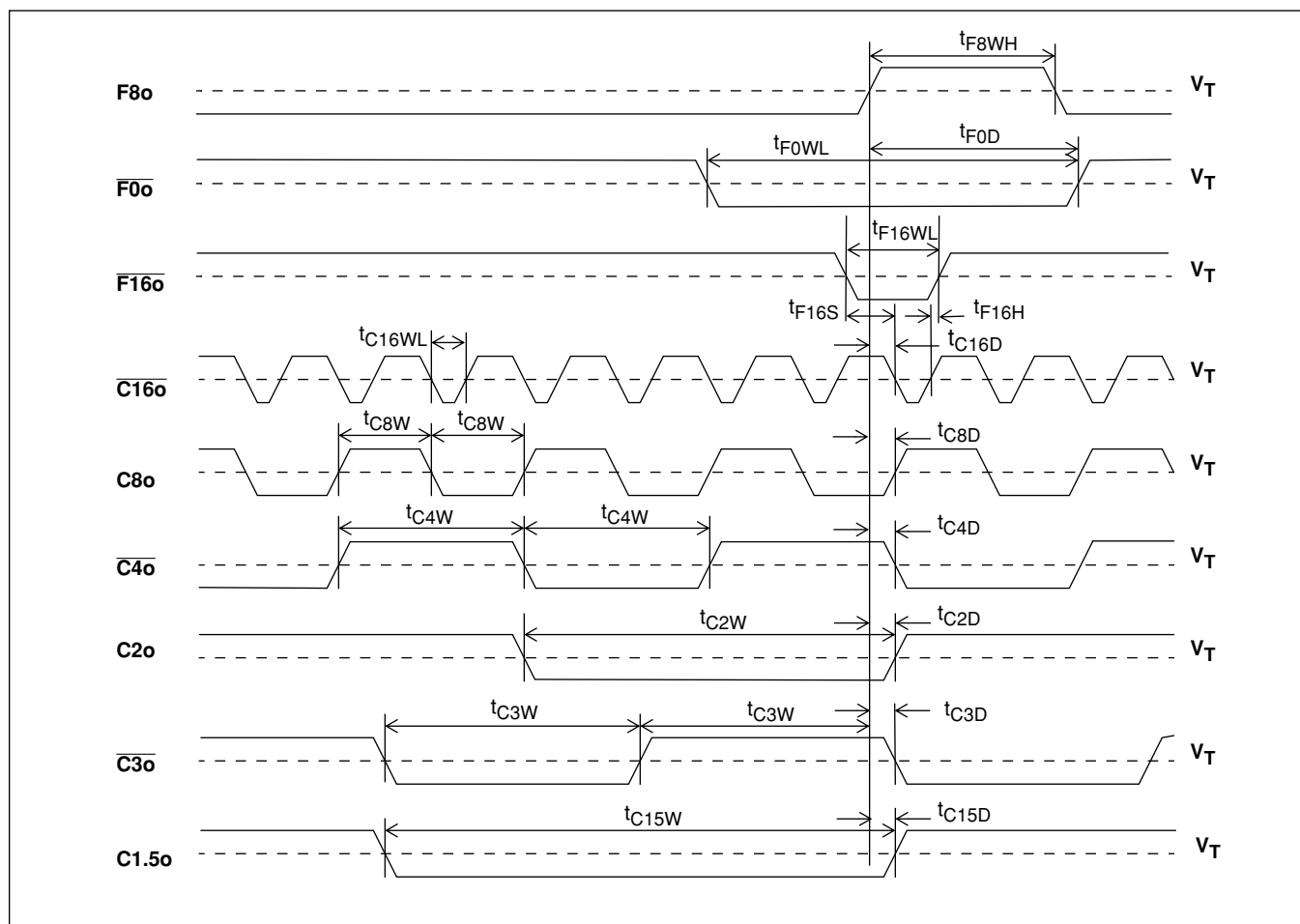
Figure 20 - Output Timing 1
