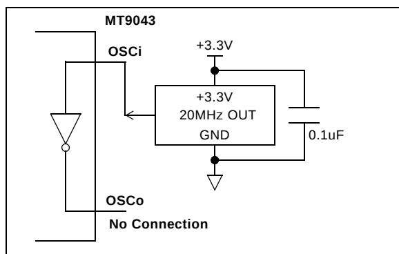
Figure 8 - Clock Oscillator Circuit
