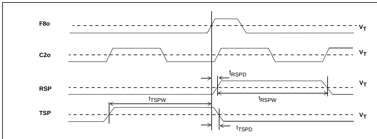
Figure 15 - Output Timing 2
