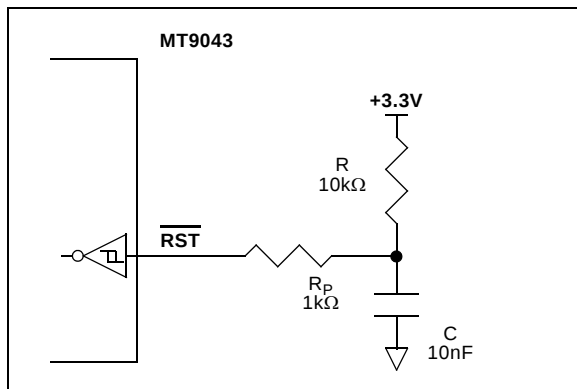
Figure 10 - Power-Up Reset Circuit
