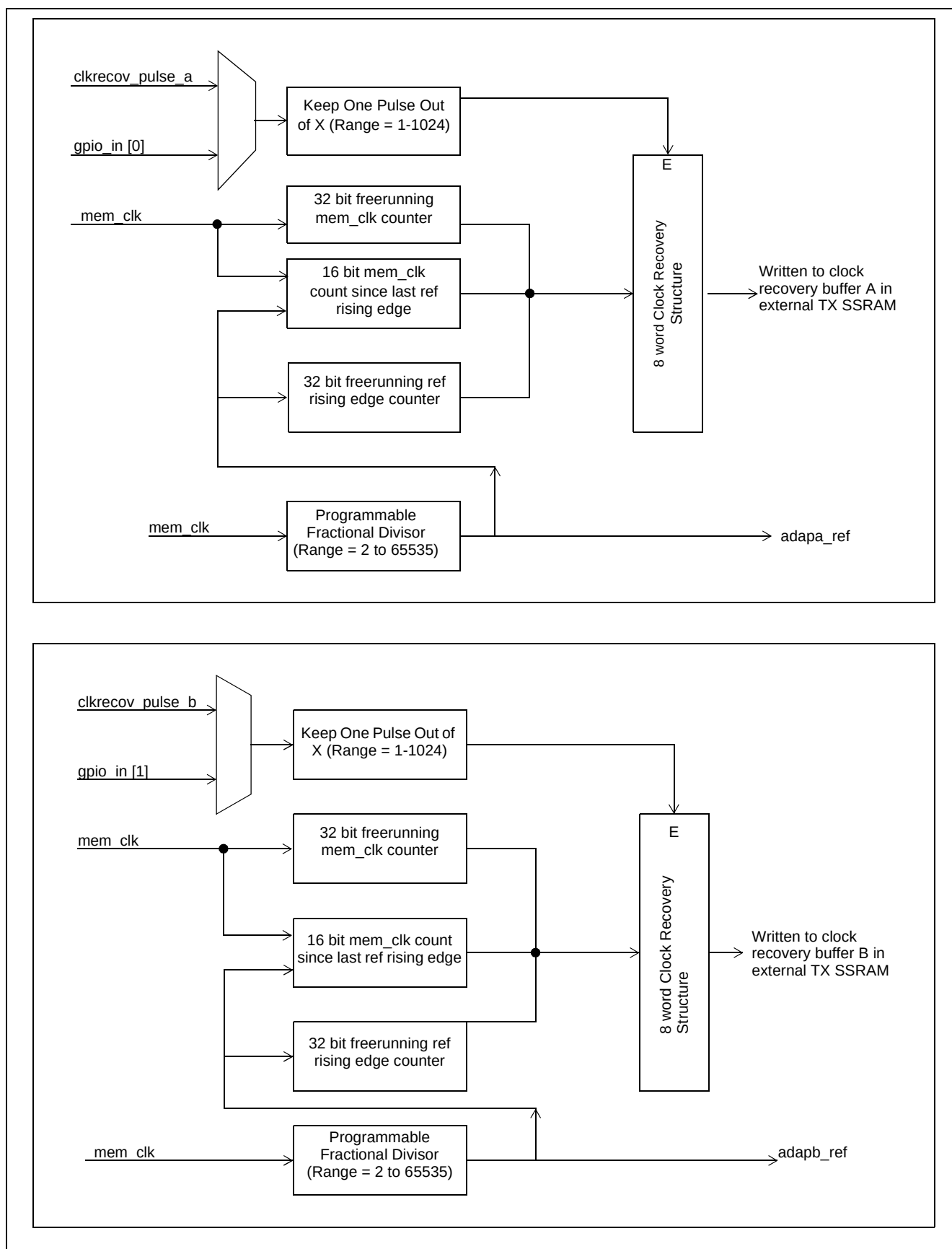
Figure 47 - Adaptive Clock Recovery Modules
