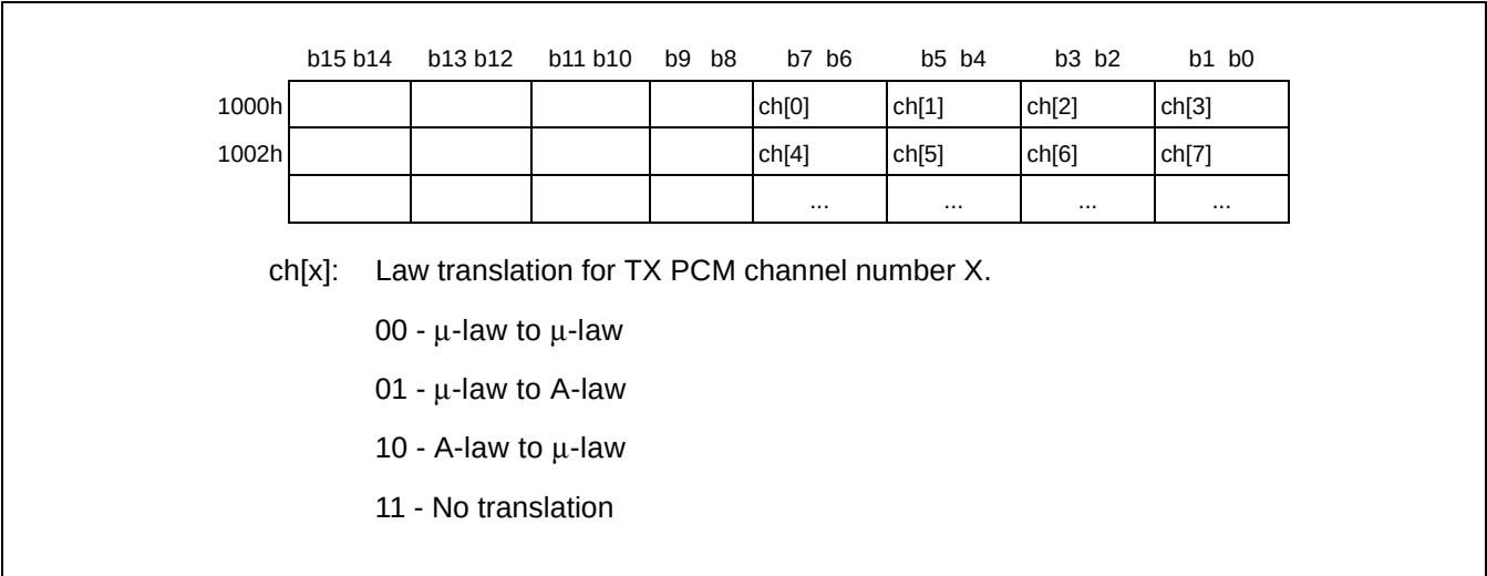
Figure 53 - PCM Law Table
