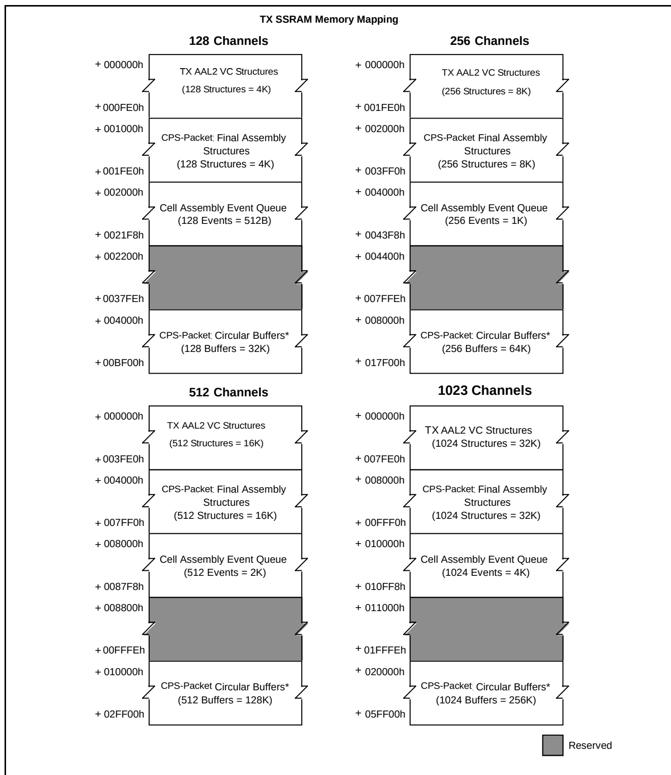
Figure 65 - TX SSRAM Memory Mapping for Fixed Structures
