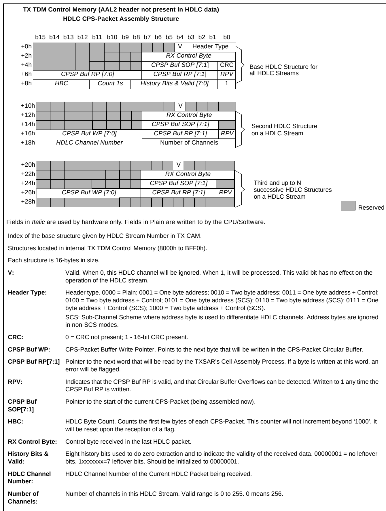
Figure 13 - HDLC CPS-Packet Assembly Structure
