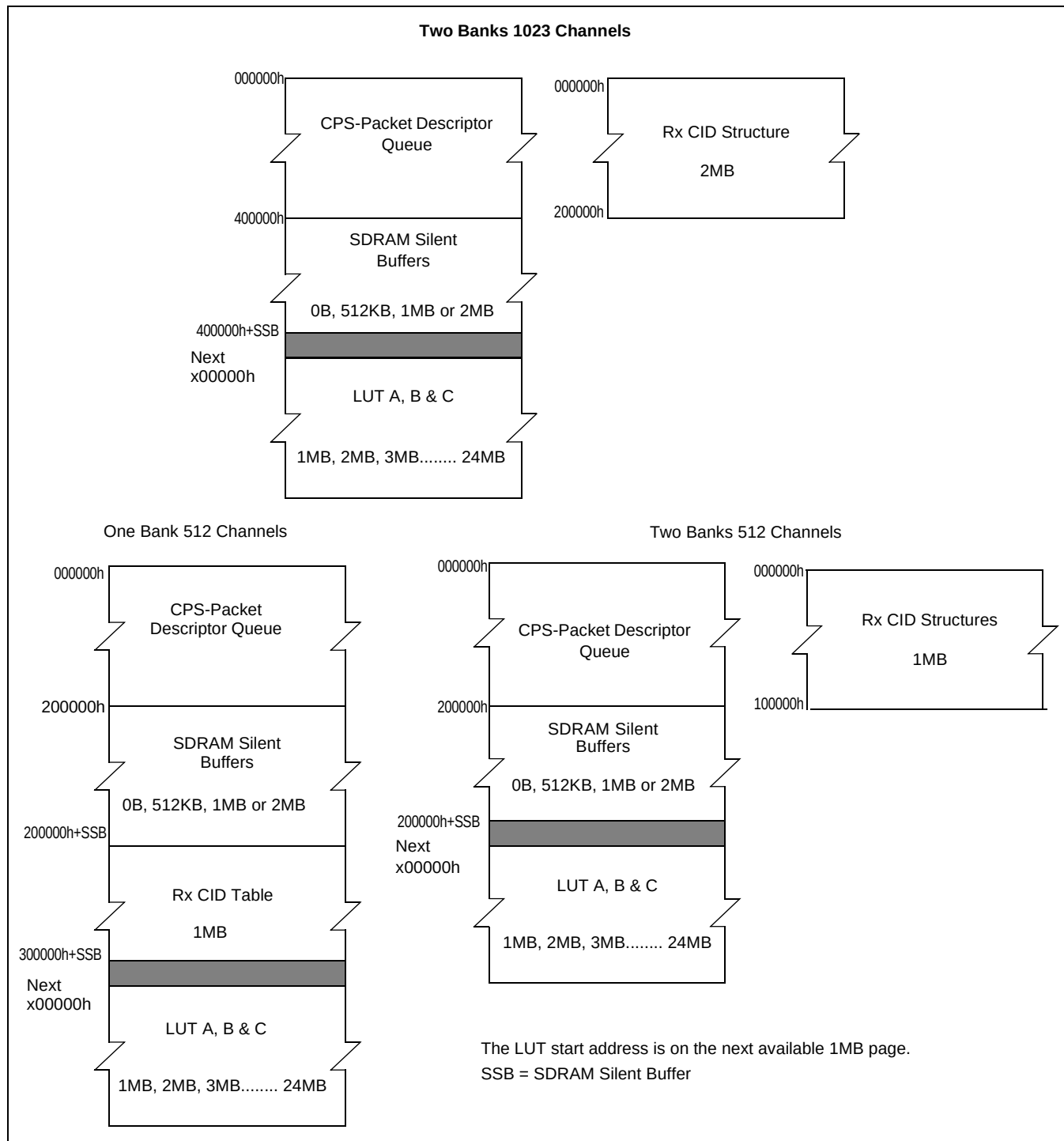
Figure 67 - SDRAM Memory Map for 512 &amp; 1023 Channels
