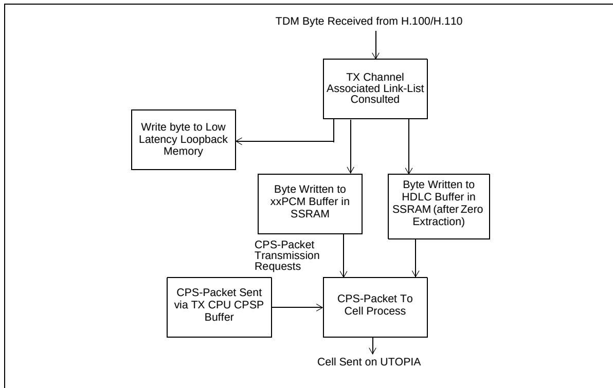
Figure 3 - TX Cell Flow
