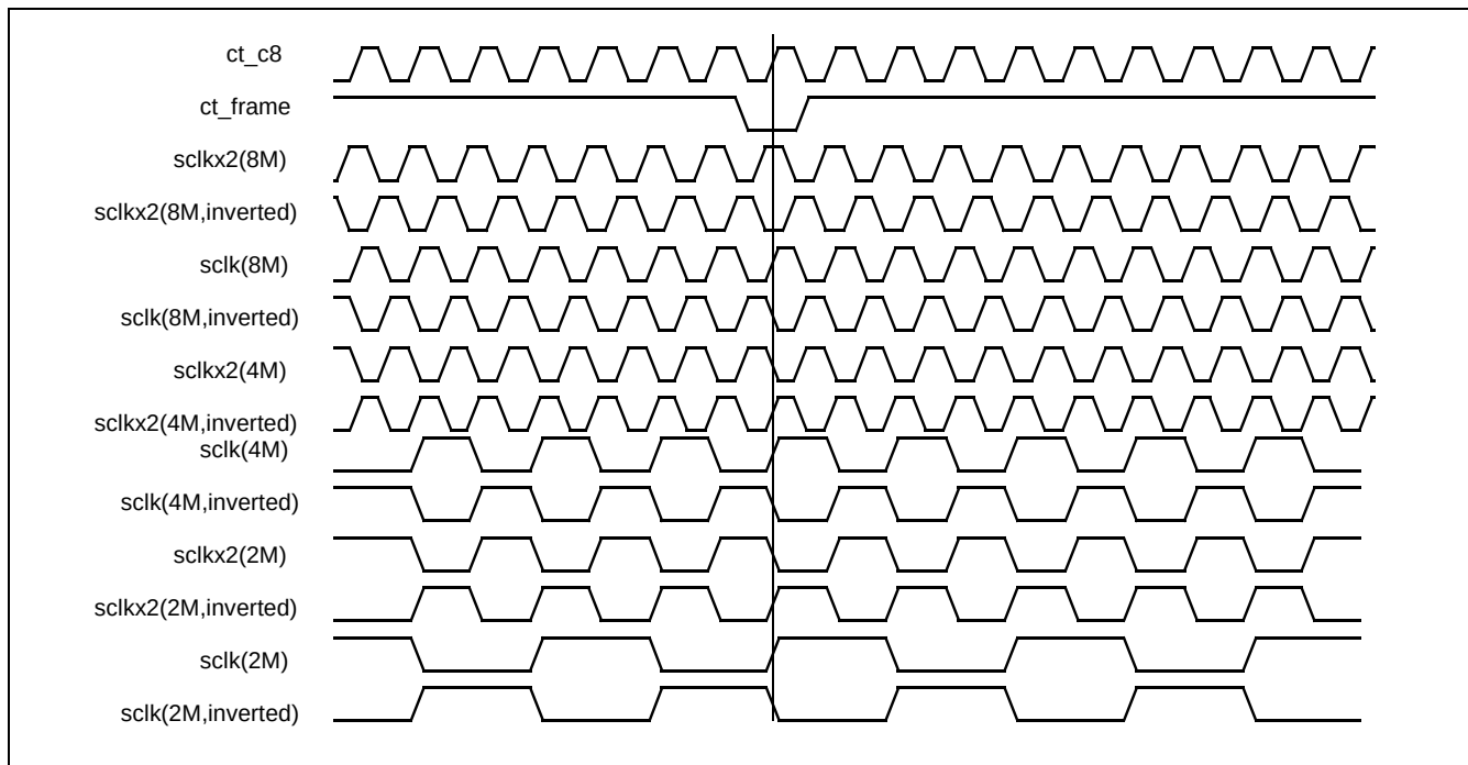
Figure 42 - TDM Bus Timing - sclx2 Generation
