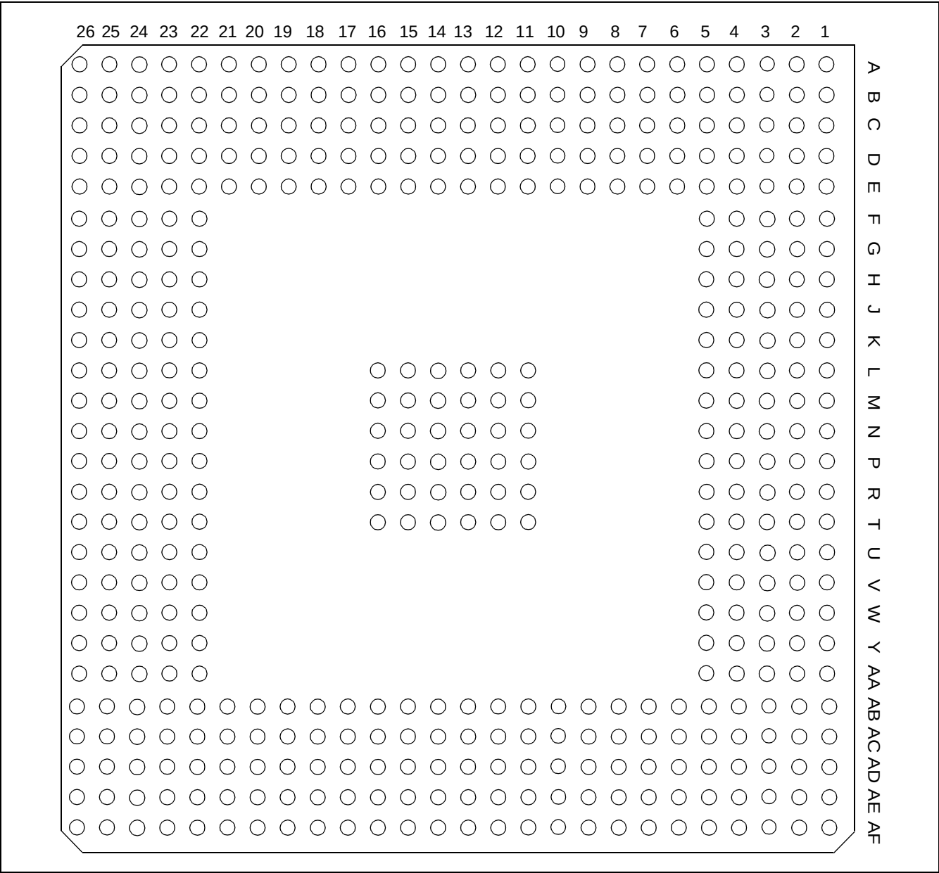
Figure 2 - 456 PBGA
