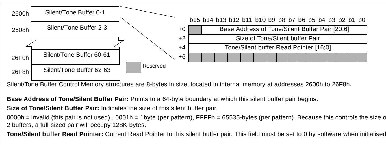
Figure 57 - SSRAM Tone Buffer Control Memory
