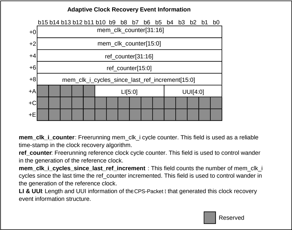
Figure 46 - Adaptive Clock Recovery Event Information
