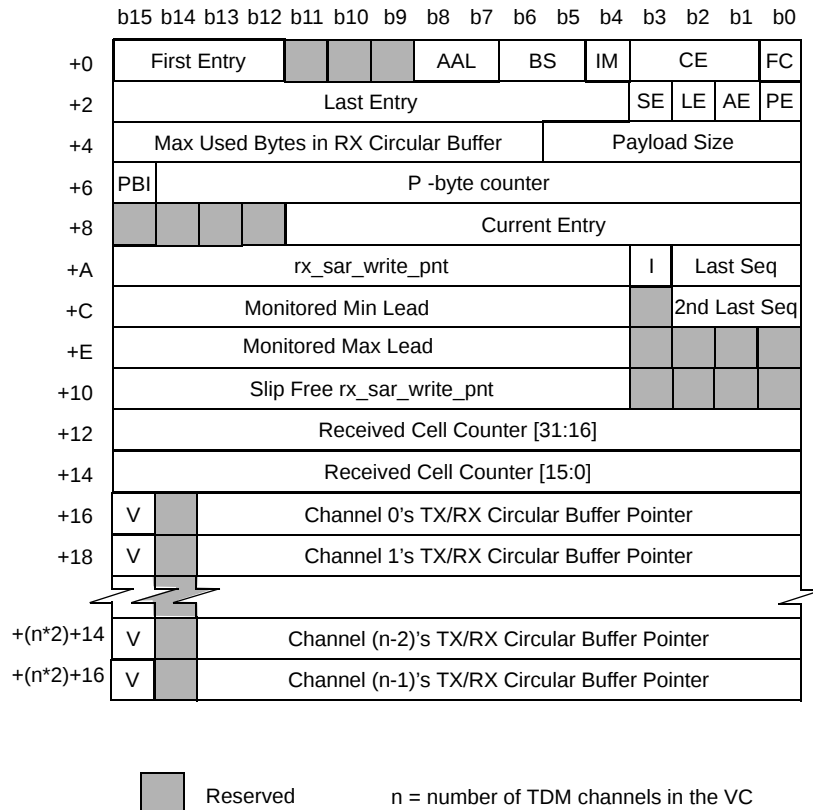
Figure 30 - RX_SAR Control Structure
