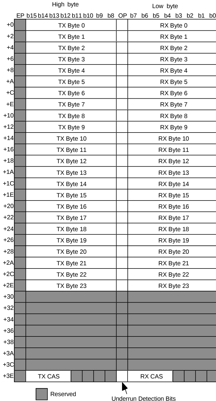
Figure 16 - TDM Circular Buffer (one MultiFrame in T1 mode)
