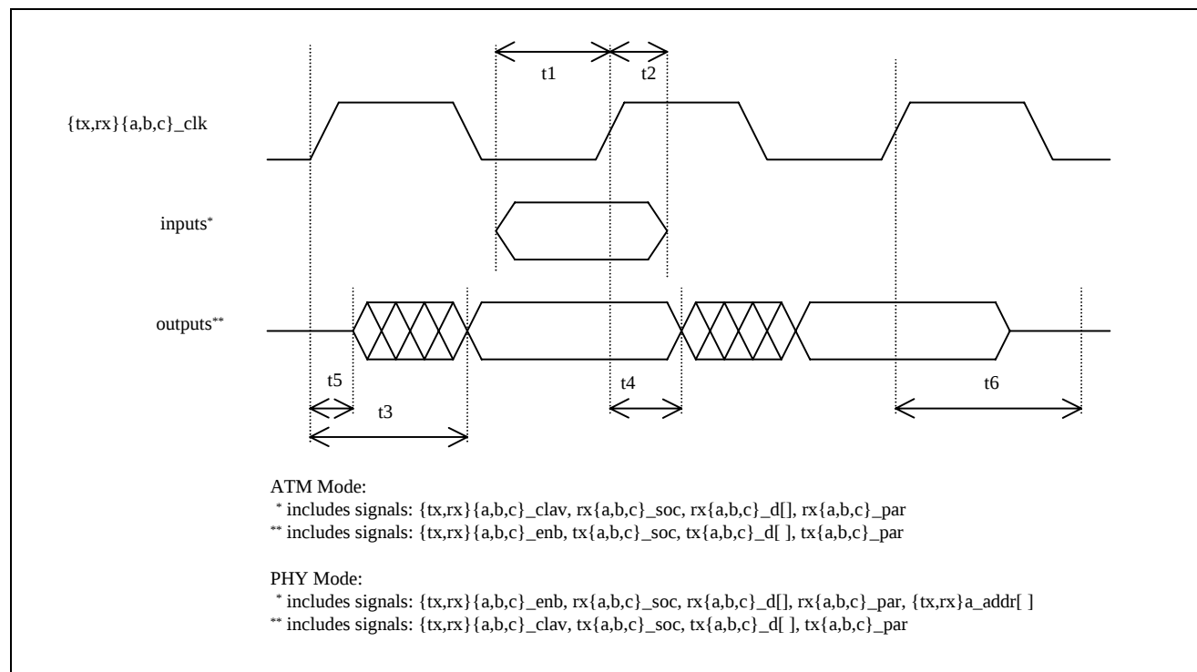
Figure 60 - UTOPIA Timing
