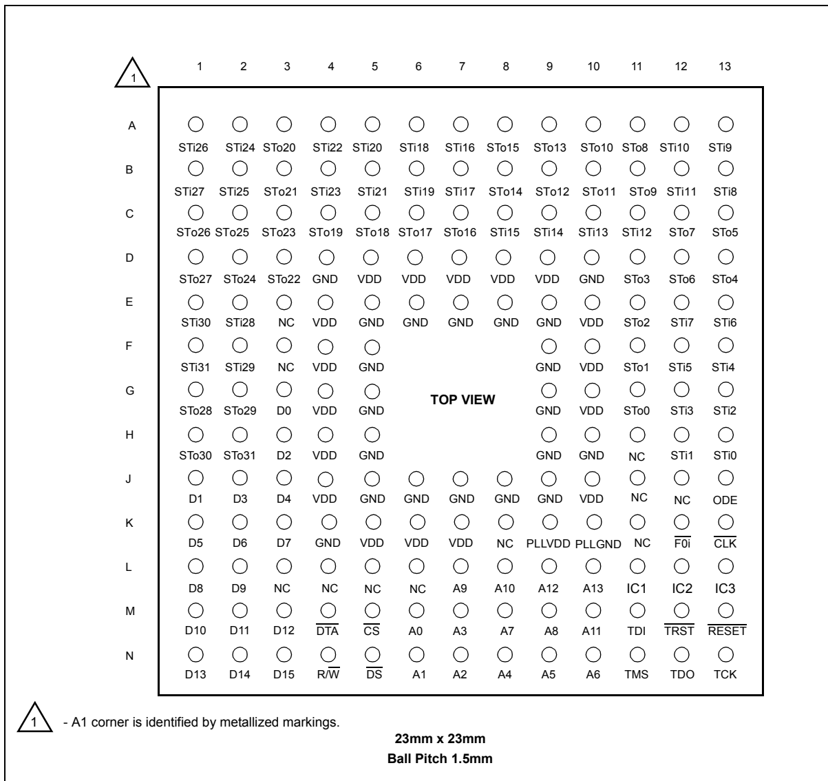
Figure 3 - 160 Ball PBGA Pin Connections
