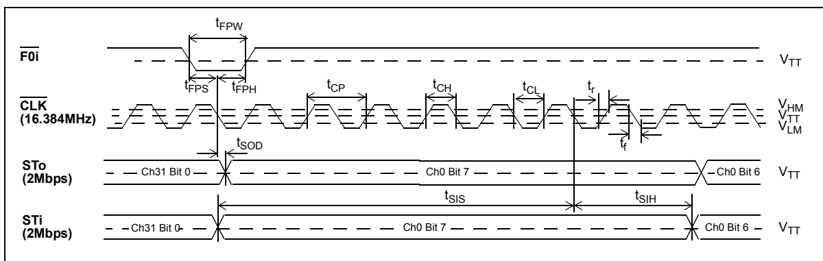
Figure 12 - ST-BUS Timing for Stream rate of 2.048Mbps when CLK = 16.384MHz
