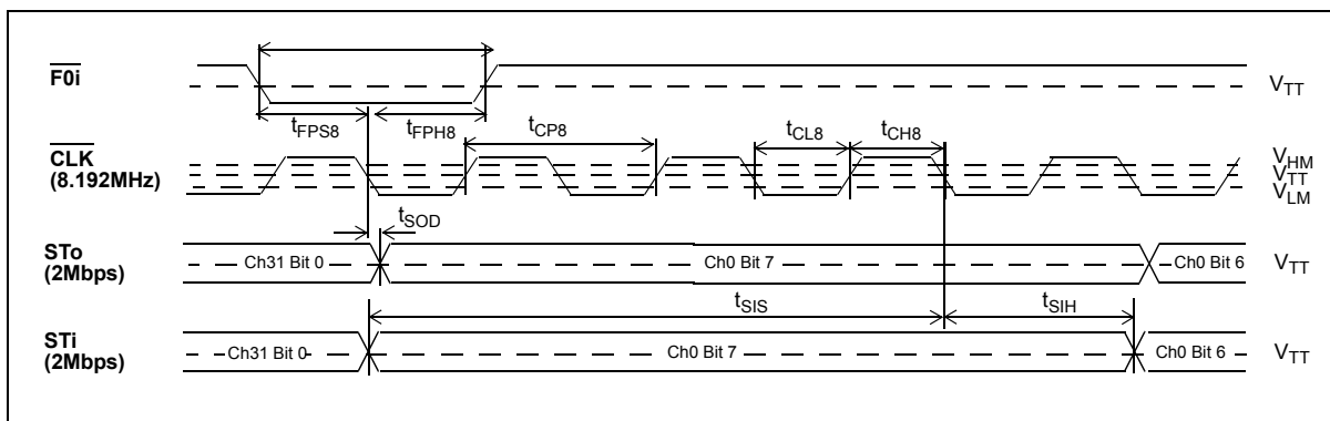
Figure 13 - ST-BUS Timing for Stream rate of 2.048Mbps when CLK = 8.192MHz
