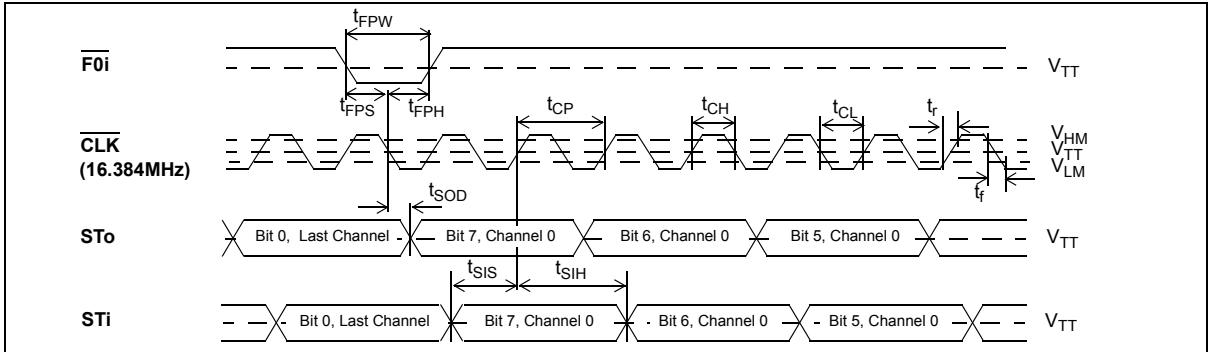
Figure 9 - ST-BUS Timing for Stream rate of 8.192Mbps
