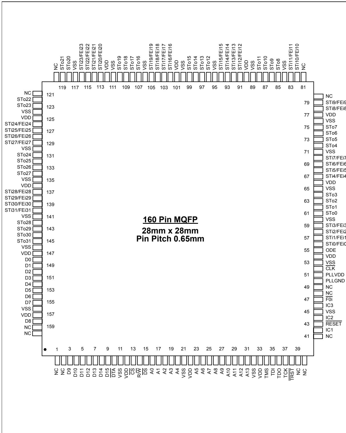
Figure 2 - 160-Pin MQFP Pin Connections
