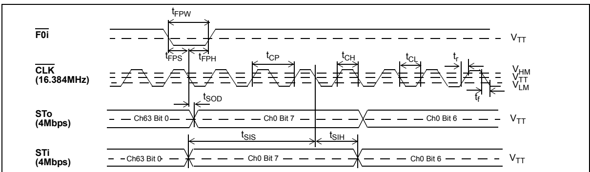
Figure 10 - ST-BUS Timing for Stream rate of 4.096Mbps when CLK = 16.384MHz
