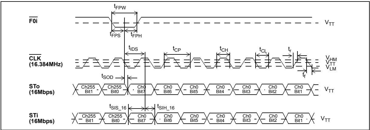
Figure 8 - ST-BUS Timing for Stream rate of 16.384Mbps
