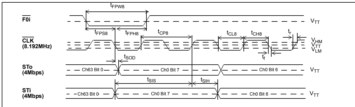
Figure 11 - ST-BUS Timing for Stream rate of 4.096Mbps when CLK = 8.192MHz
