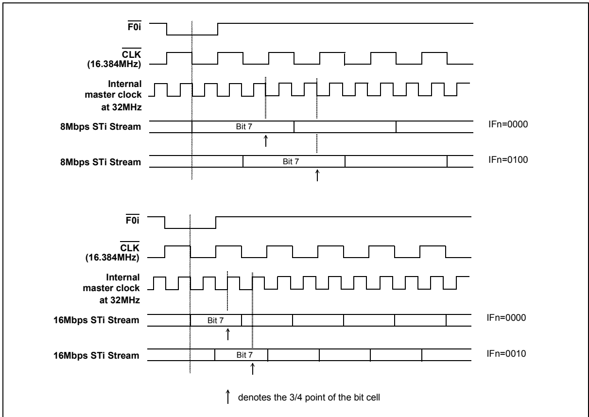
Figure 6 - Examples for Input Offset Delay Timing
