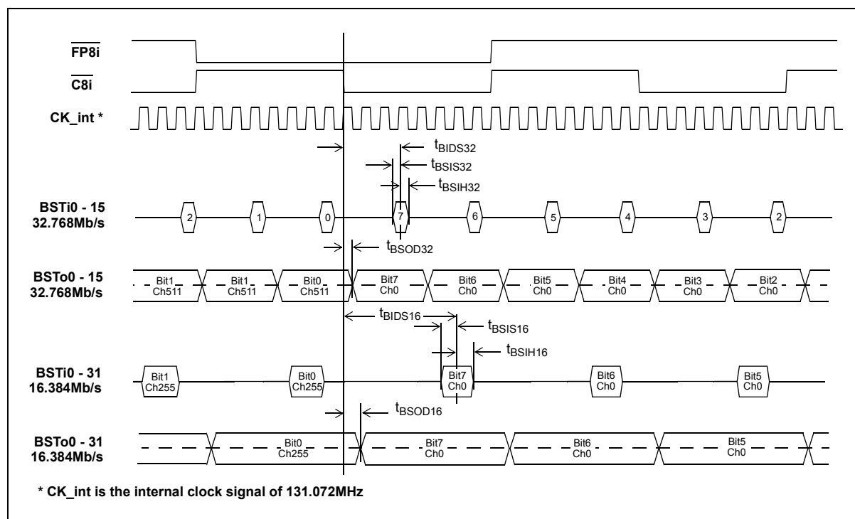
Figure 23 - ST-BUS Backplane Data Timing Diagram (32Mb/s, 16Mb/s)
