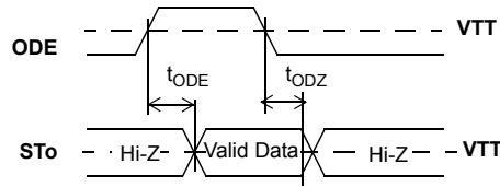
Figure 29 - Output Driver Enable (ODE)
