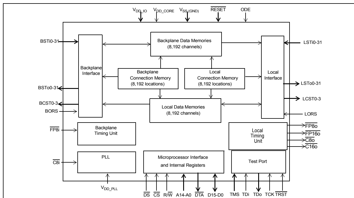
Figure 1 - MT90869 Functional Block Diagram
