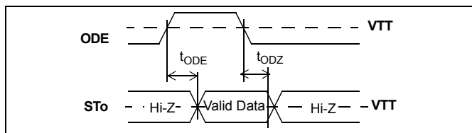
Figure 28 - Output Driver Enable (ODE)
