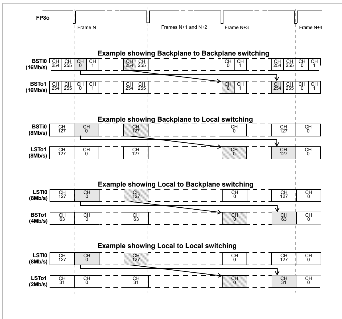
Figure 15 - Constant Switch Delay: Examples of different stream rates and routing
