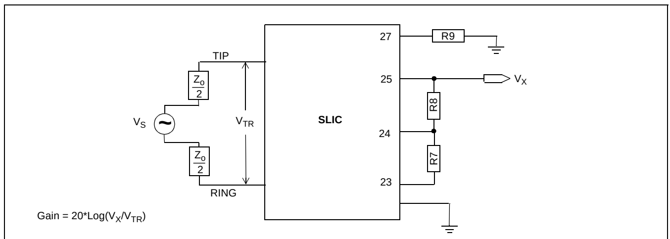
Figure 9 - 2-4 Wire Gain
