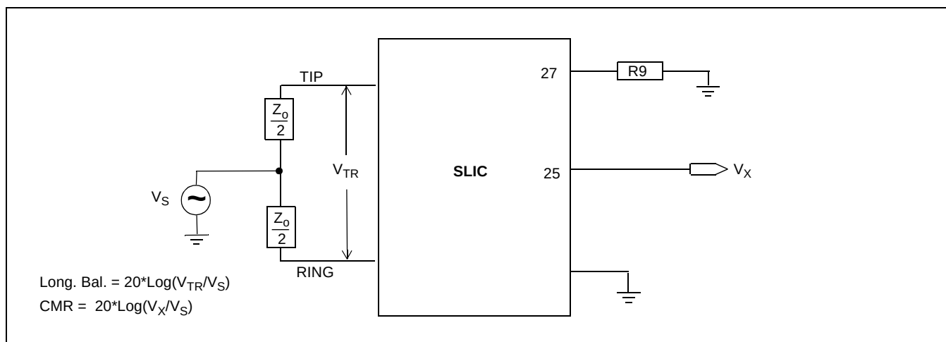
Figure 11 - Longitudinal Balance &amp; CMR
