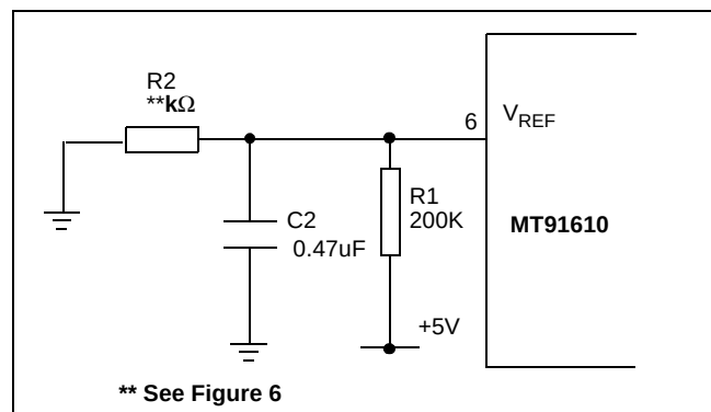
Figure 3 - Loop Setting
