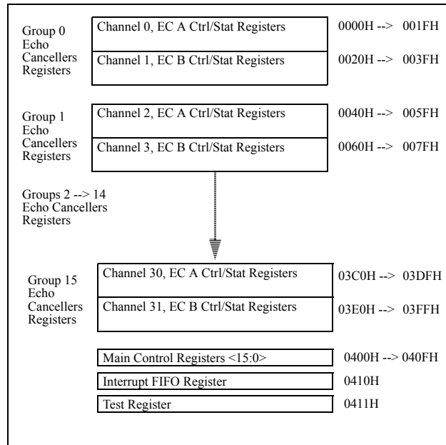
Figure 9 - Memory Mapping
