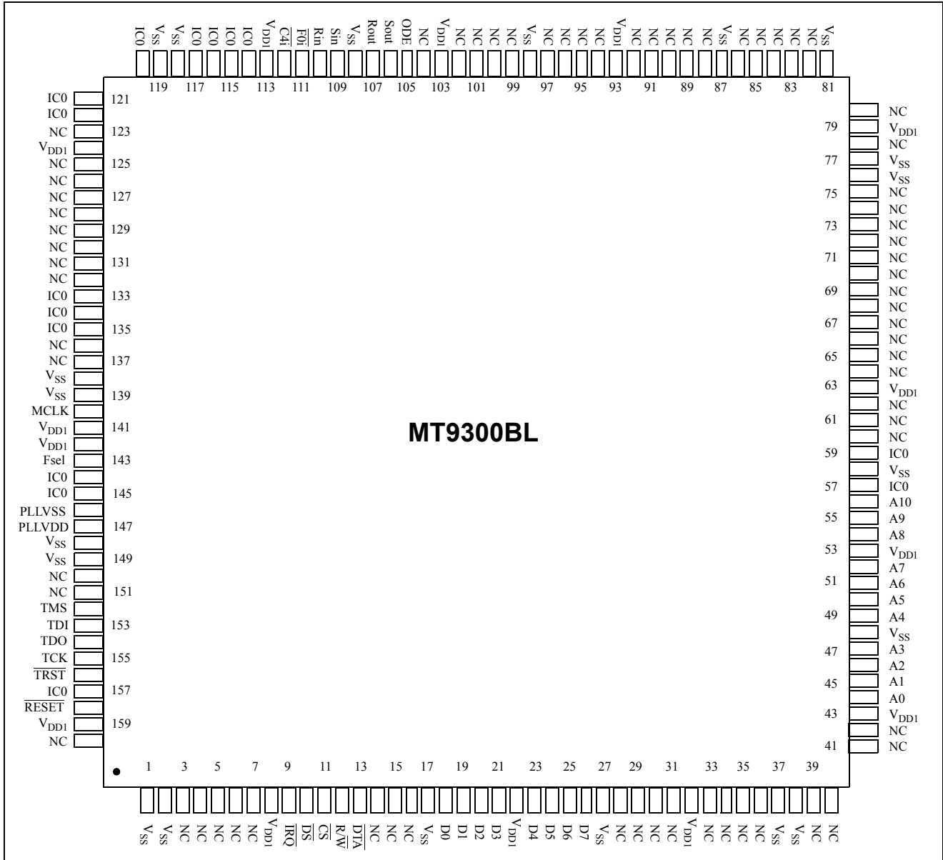
Figure 3 - 160 Pin MQFP
