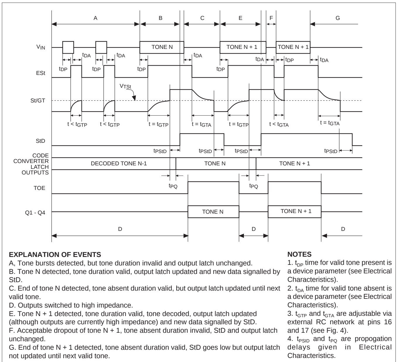
Figure 5: Timing diagram
