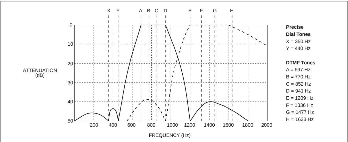
Figure 3: Filter response
