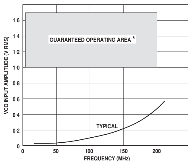
Fig. 3 Input sensitivity
