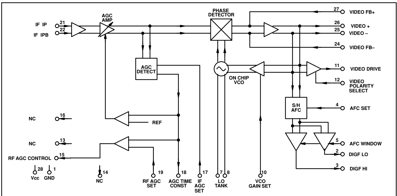
Fig. 2 Block diagram
