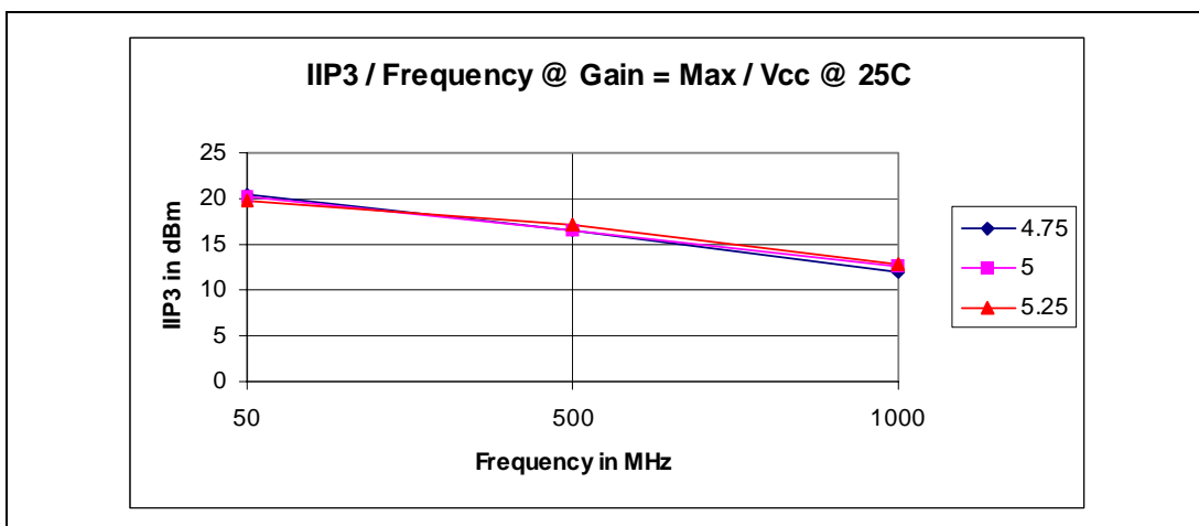
Figure 26 - Typical Out1, Out2 & Out3 IIP3 / Frequency @ Gain = Max / Vcc @ 25C
