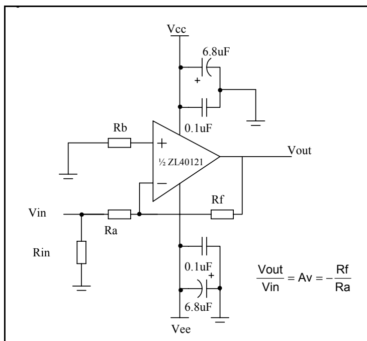
Figure 3 - Inverting Gain
