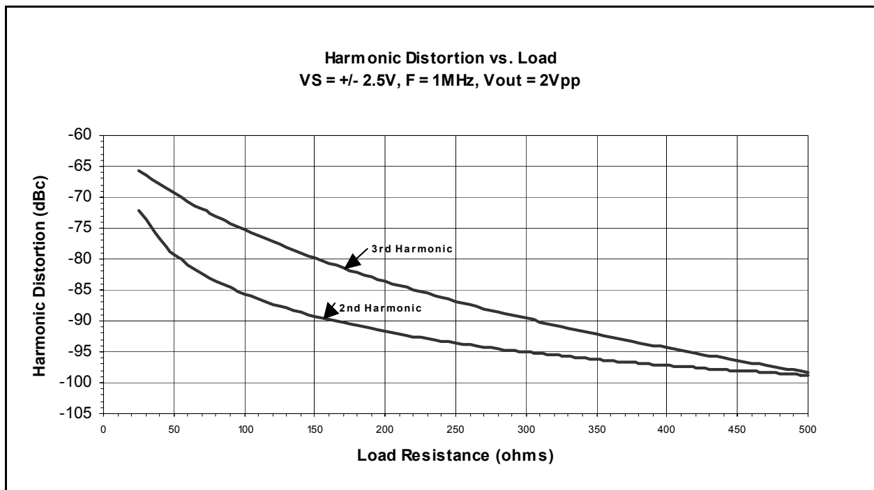
Figure 25 - Harmonic Distortion vs. Load VS = \pm 2.5\text{V} , F = 1MHZ, Vout = 2Vpp
