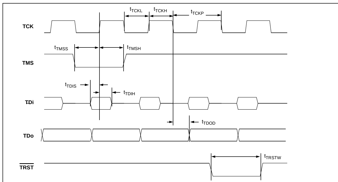
Figure 34 - JTAG Test Port Timing Diagram
