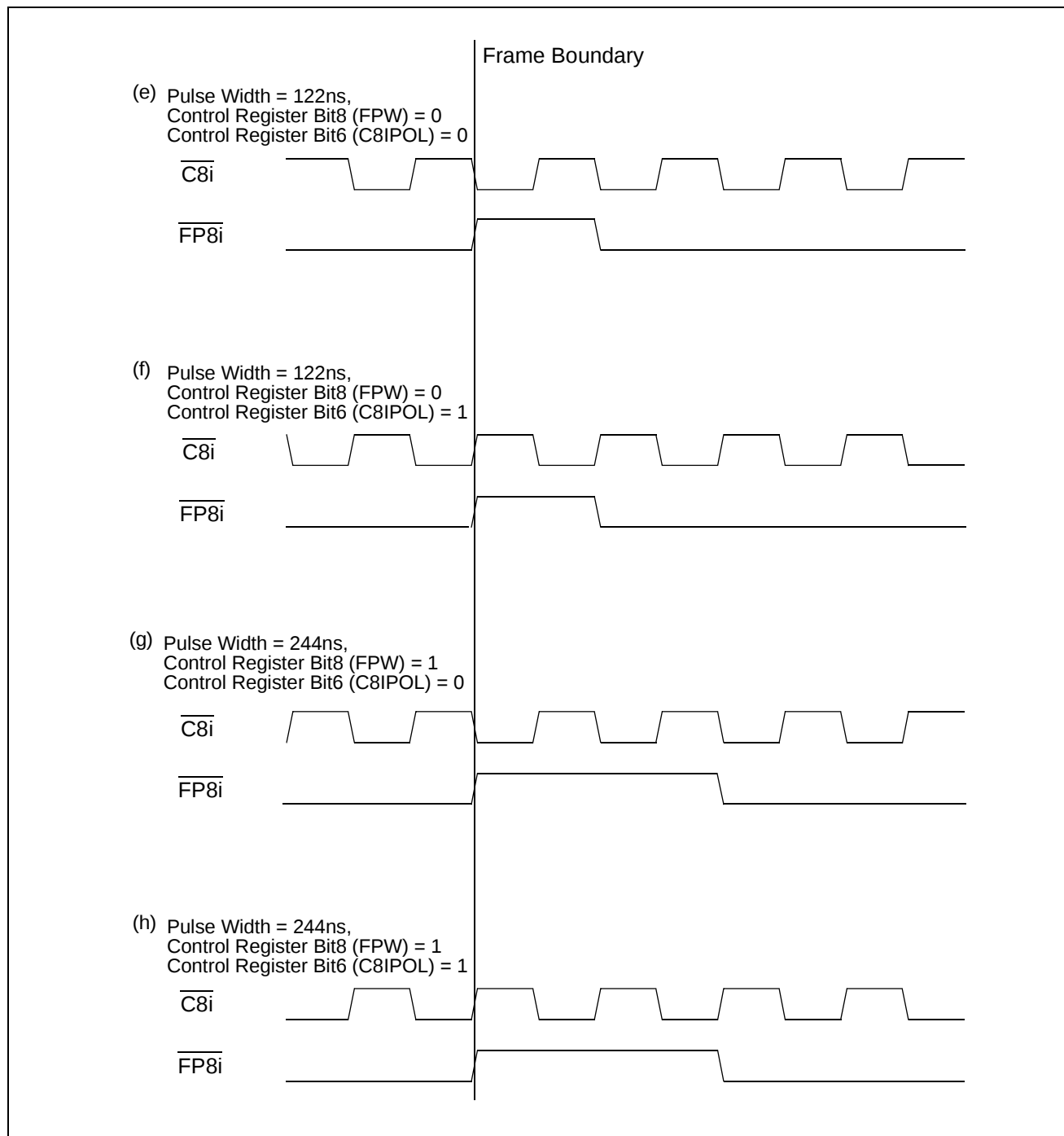
Figure 24 - Frame Boundary Conditions, GCI-Bus Operation
