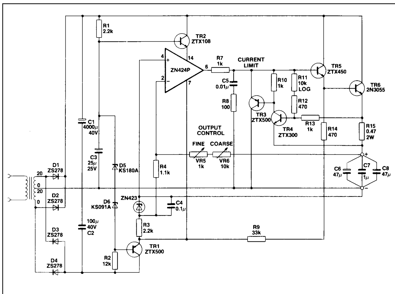
Fig.7 0V to 12V, 1A power supply
