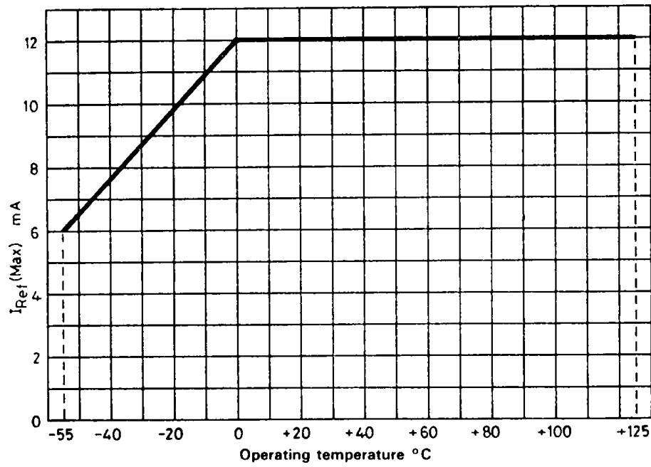
Fig.3 Derating curve
