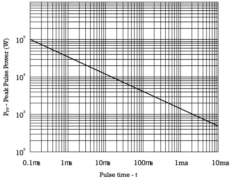
PEAK PULSE POWER RATING CURVE
