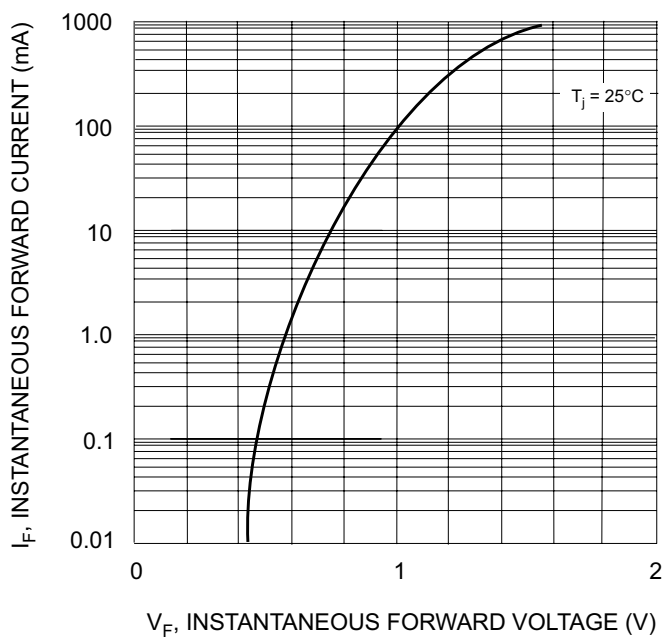
Fig. 1 Forward Characteristics
