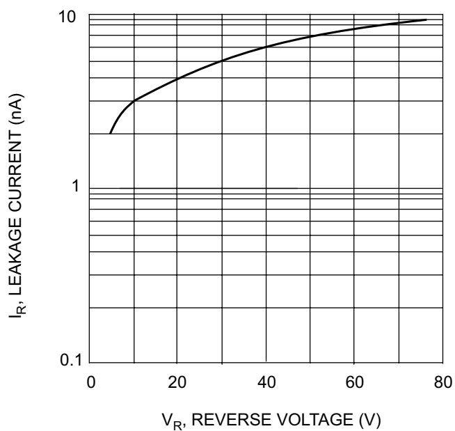
Fig. 2 Typical Leakage Current vs Reverse Voltage
