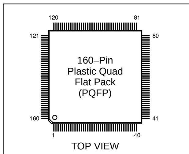
Figure A. Pin Configuration
