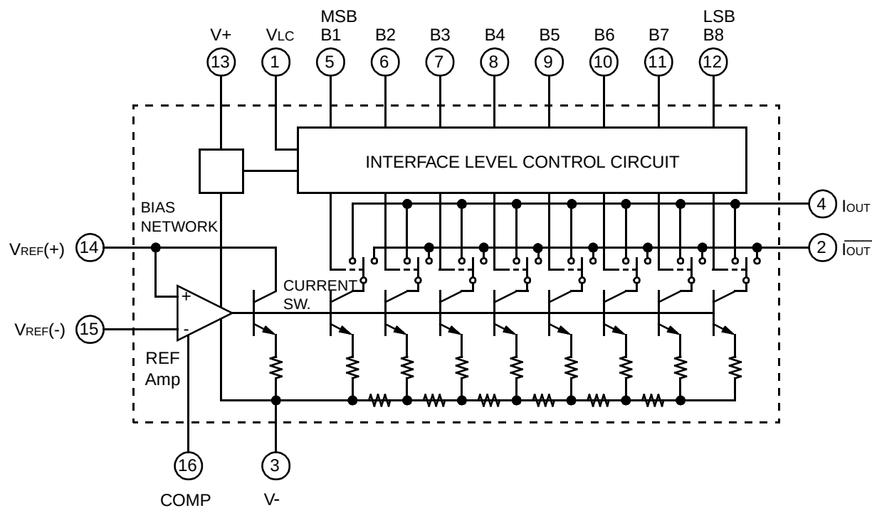
Fig. 1 - BLOCK DIAGRAM
