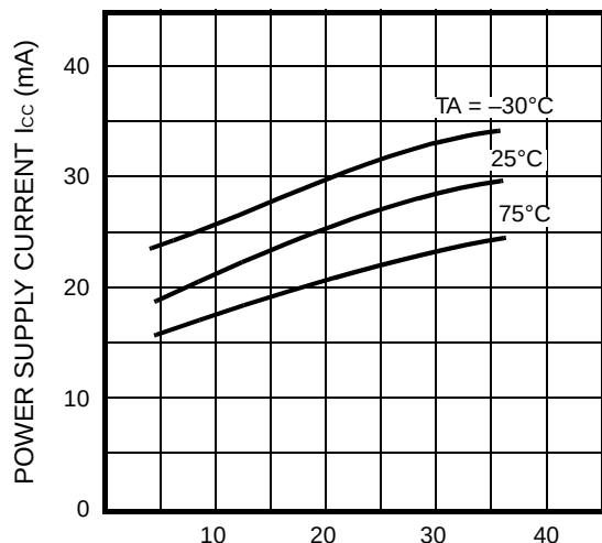
Figure 2 POWER SUPPLY CURRENT vs POWER SUPPLY VOLTAGE
