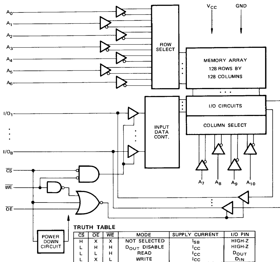
Fig. 1 – MB 8128 BLOCK DIAGRAM
