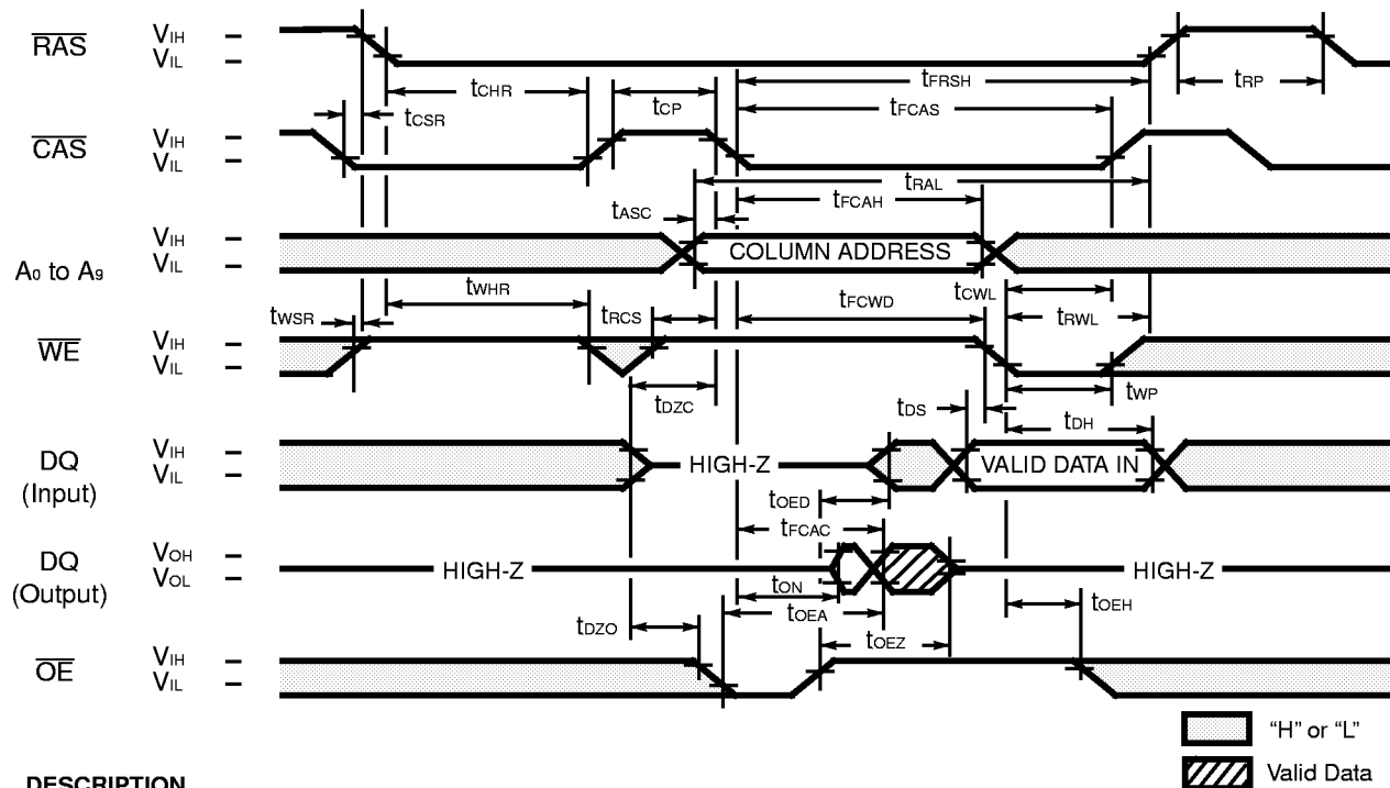
Fig. 20 – \overline{\text{CAS}}\text{-BEFORE-}\overline{\text{RAS}} REFRESH COUNTER TEST CYCLE
