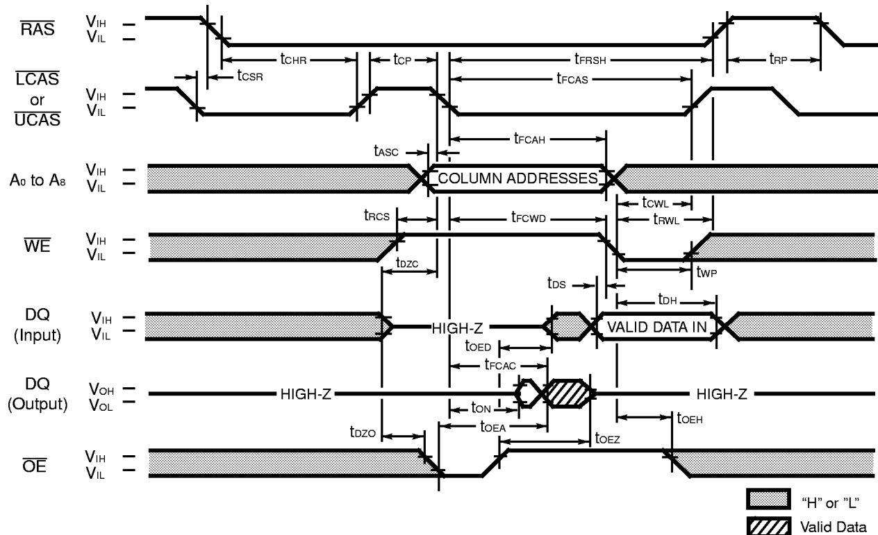
Fig. 19 – \overline{\text{CAS}}\text{-BEFORE-}\overline{\text{RAS}} REFRESH COUNTER TEST CYCLE
