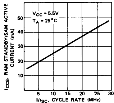
Fig. 21 – RAM STANDBY/SAM ACTIVE CURRENT vs CYCLE RATE
