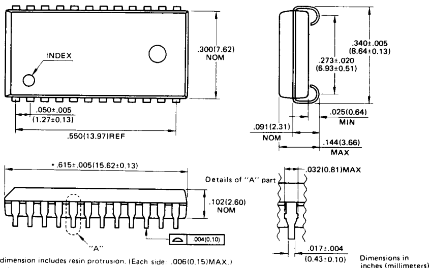
24-LEAD PLASTIC LEADED CHIP CARRIER (CASE No.: LCC-24P-M02)
