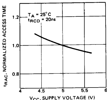
Fig. 5 — NORMALIZED ACCESS TIME vs SUPPLY VOLTAGE
