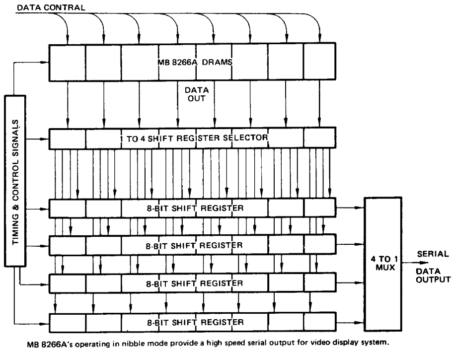
Fig. 3 – VIDEO DISPLAY SYSTEM EXAMPLE
