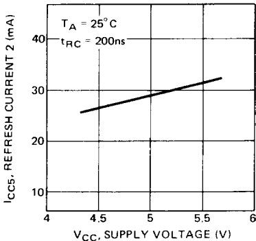
Fig. 19 — REFRESH CURRENT 2 vs SUPPLY VOLTAGE
