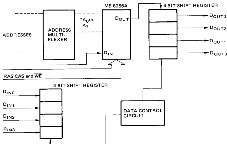
Fig. 2 – EXAMPLE OF 16K x 4 DRAM WITH MB 8266A
