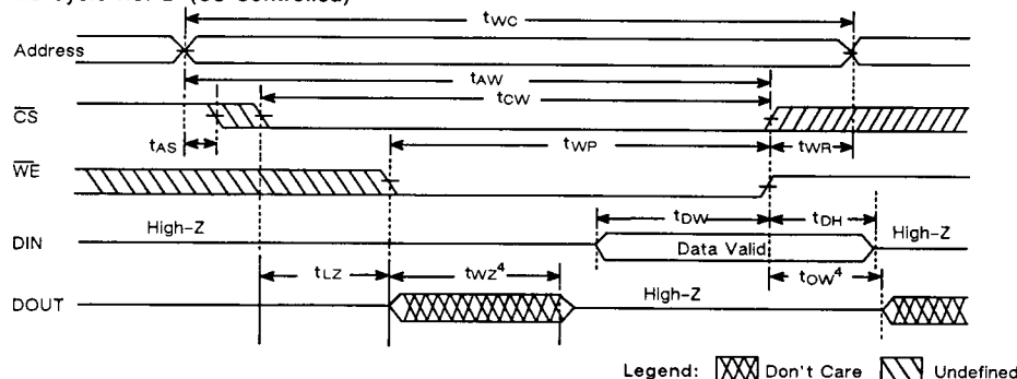
Write Cycle No. 2 ( \overline{CS} Controlled) 1,2,3
