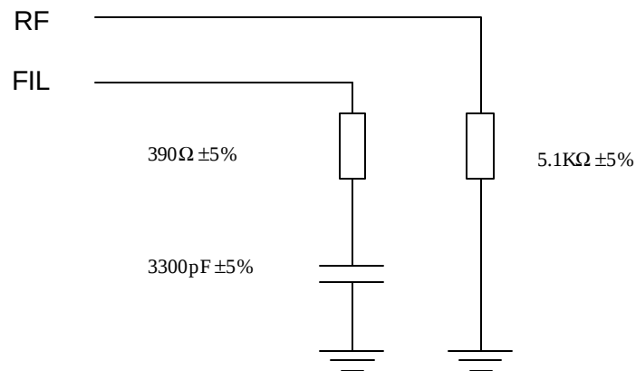
Figure 12.3 Recommended connection for build-in PLL loop filter
