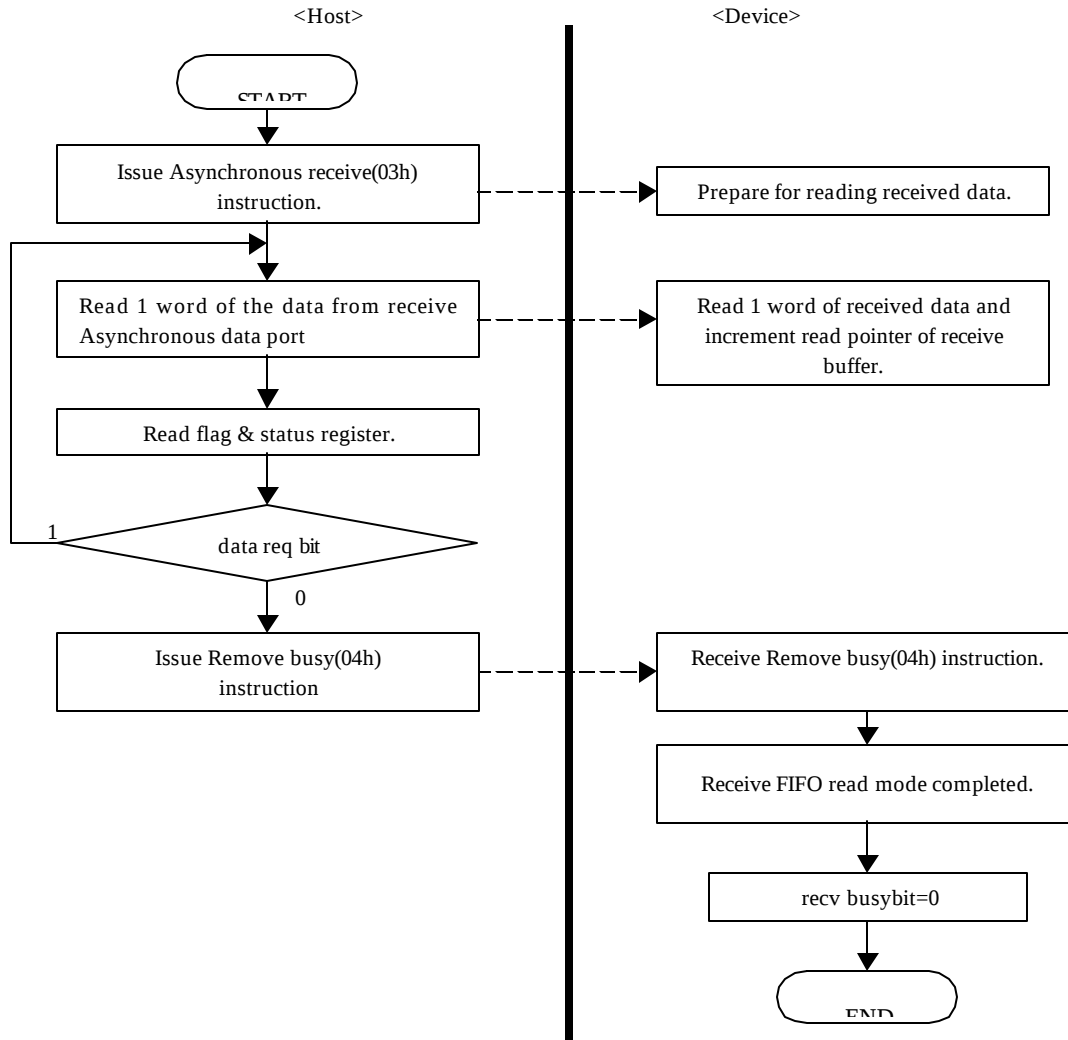
Figure 11.4.2 Flow chart for received data after storing in Asynchronous receive FIFO
