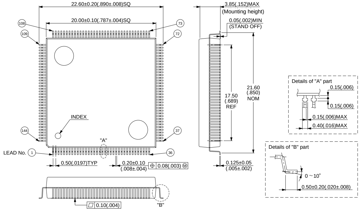
144-pin Plastic QFP (FPT-144P-M03)
