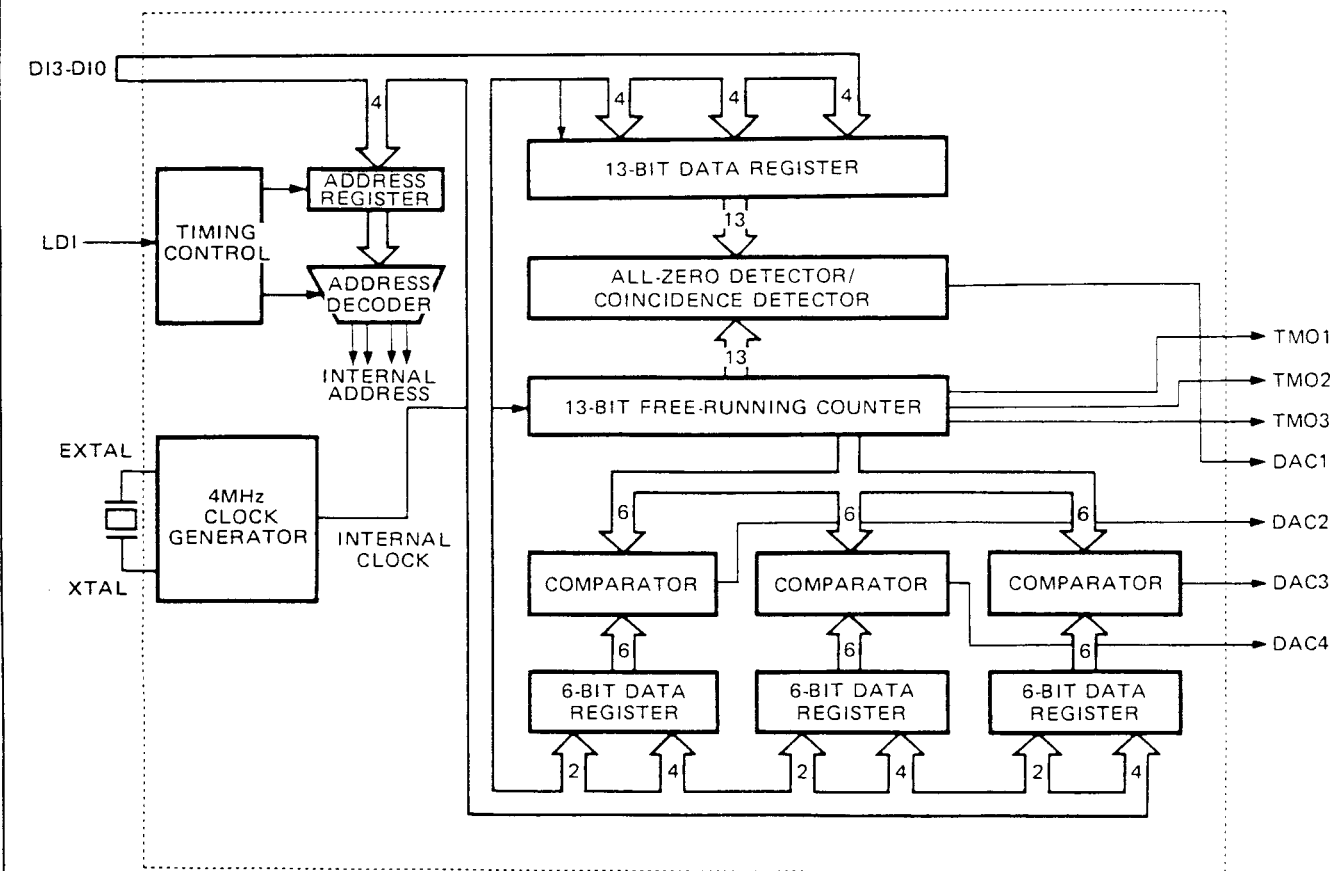
Fig. 2 – BLOCK DIAGRAM
