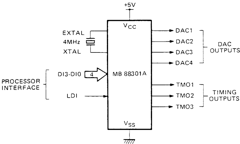
Fig. 1 – LOGIC SYMBOL
