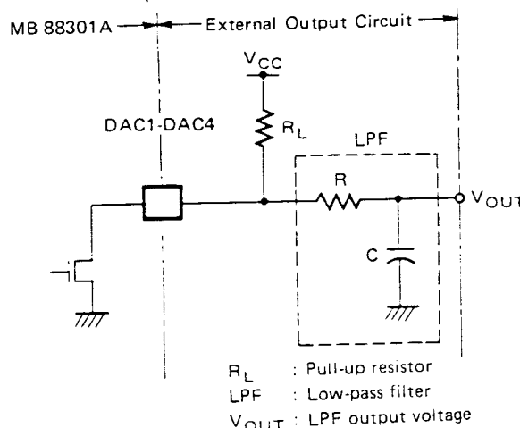
Fig. 11 — OUTPUT CIRCUIT CONFIGURATION (EXAMPLE)
