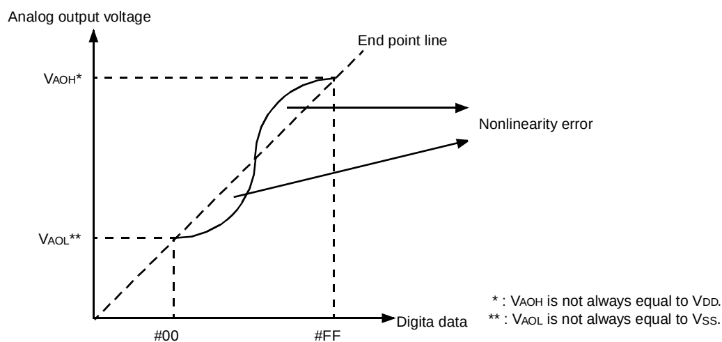
Figure 8 Definition of Nonlinearity Error
