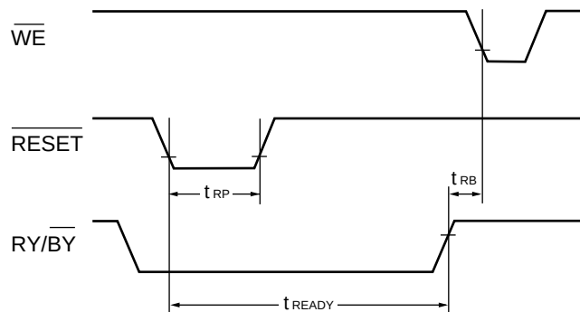
Figure 12 \overline{\text{RESET}} Timing Diagram
