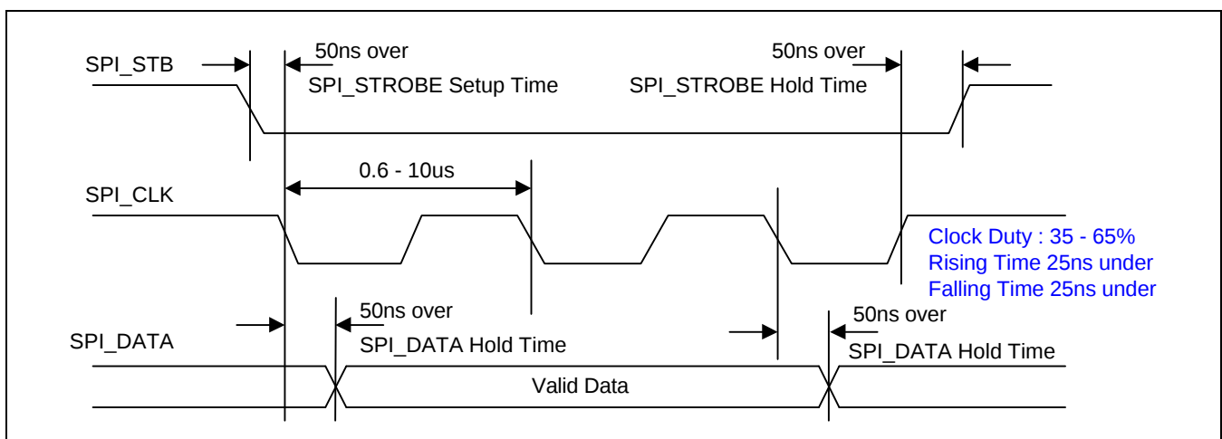
Figure 3. 3-Line Serial Port Interface Timing
