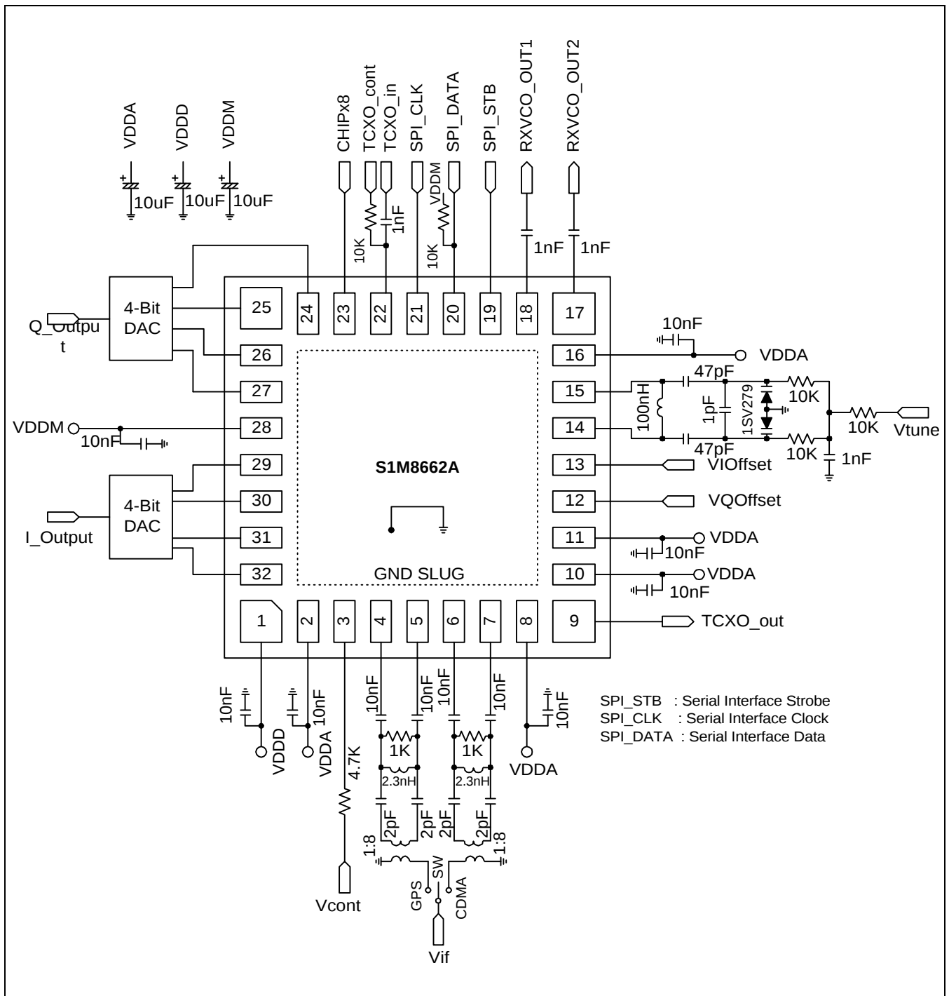
Figure 12. Test Circuit
