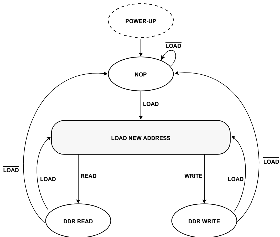
STATE DIAGRAM
