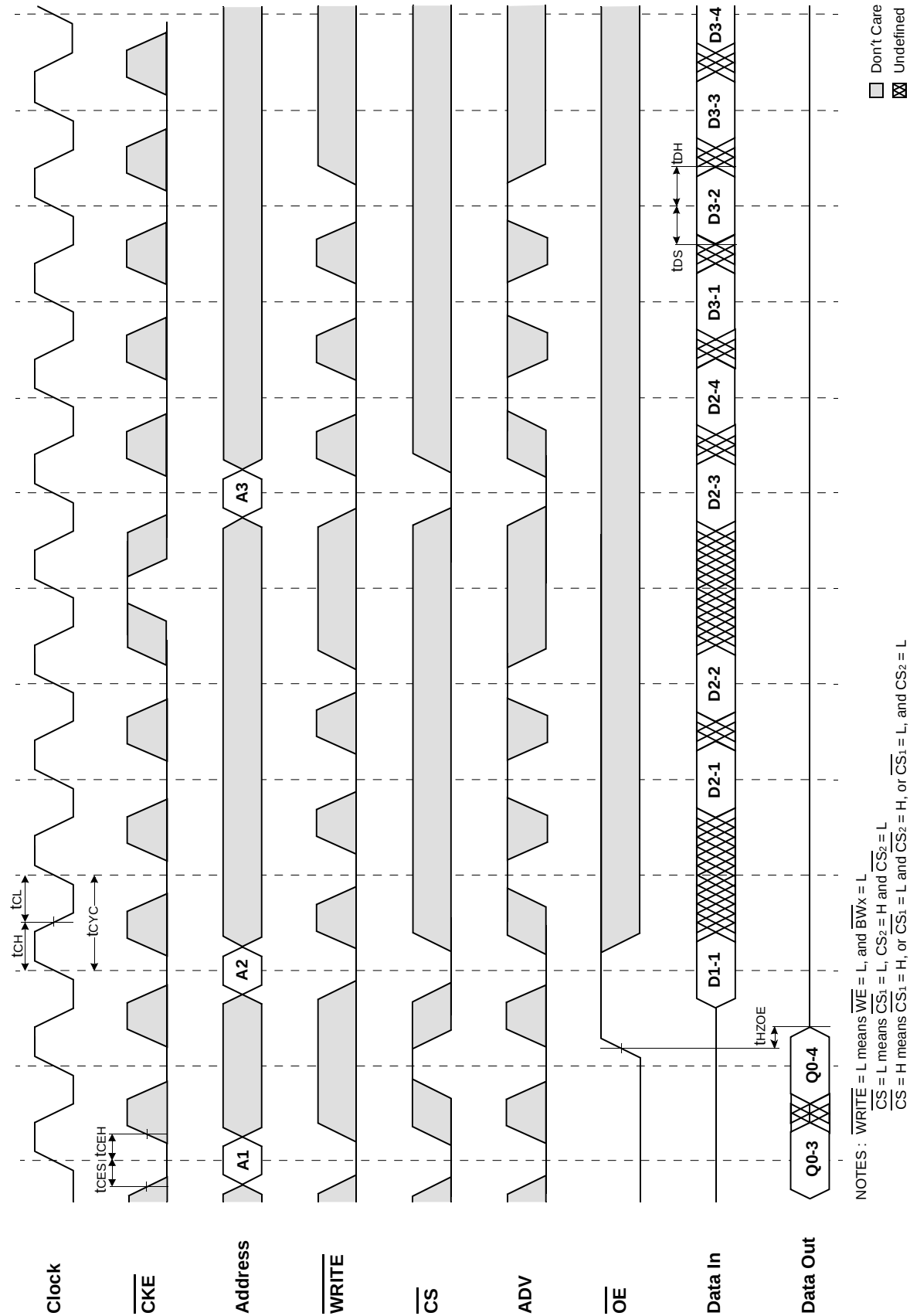
TIMING WAVEFORM OF WRITE CYCLE
