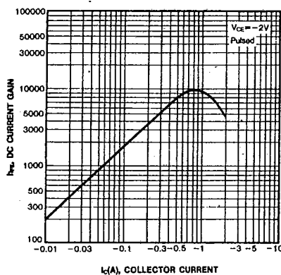
I_C(A) , COLLECTOR CURRENT
