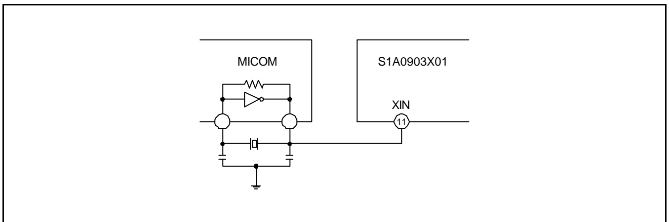
Figure. 20 Connection X'tal for Micro-processor
