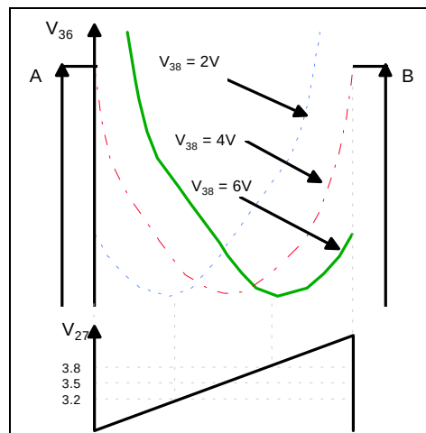
Figure 2. Keystone Adjustment
