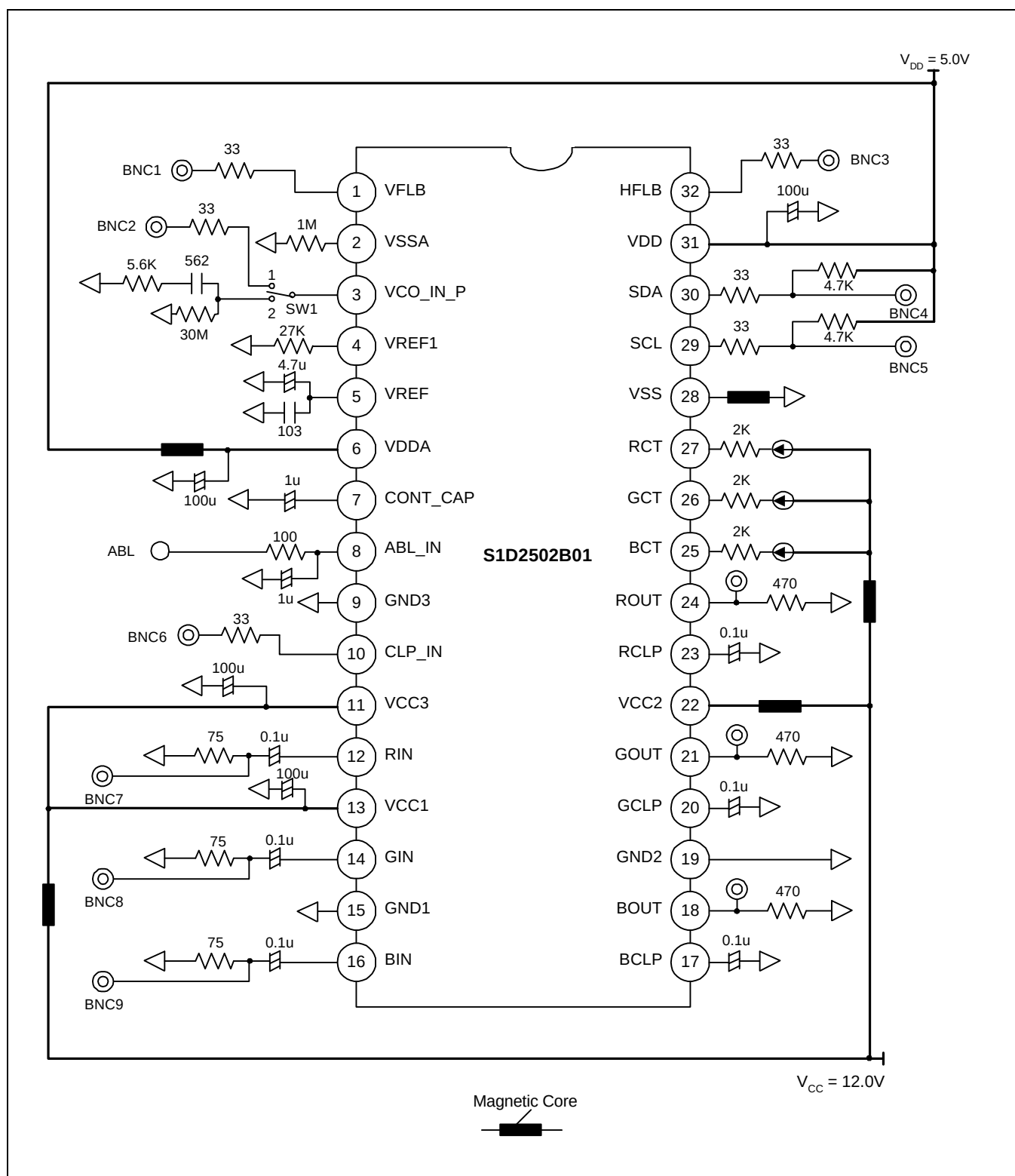
Figure 4. Test Circuit
