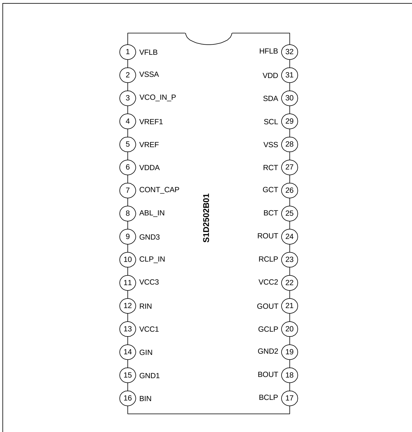
Figure 2. Pin Configuration
