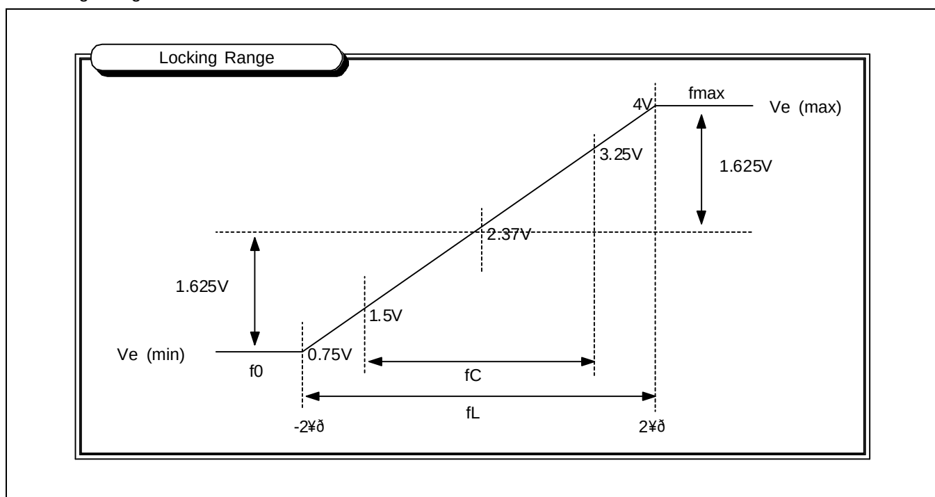
Figure 25. Locking Range
