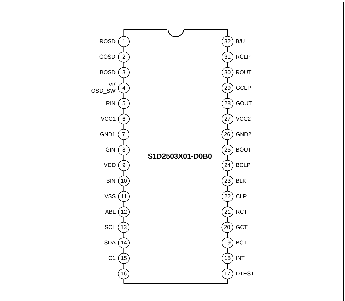
Figure 2. Pin Configuration
