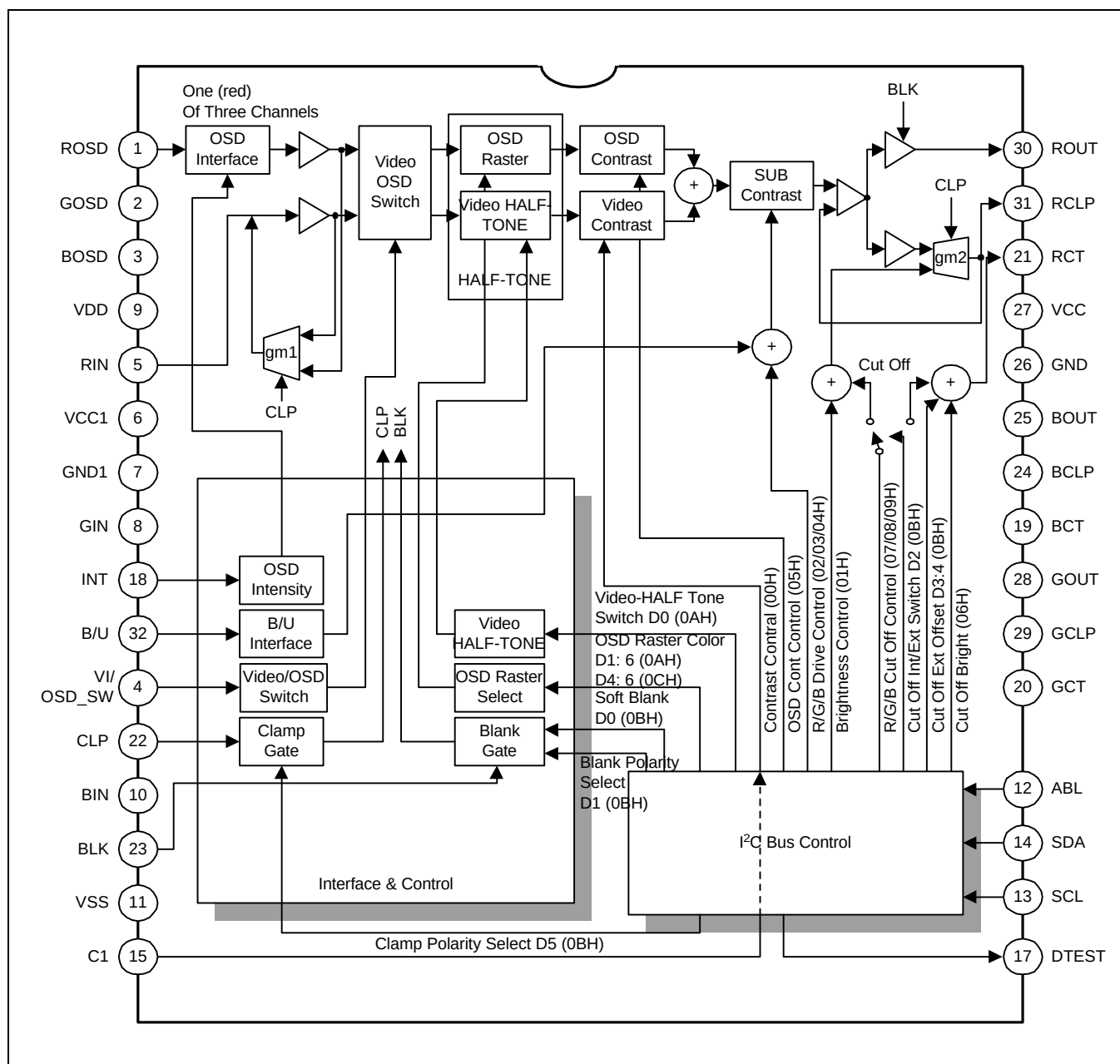
Figure 1. Block Diagram
