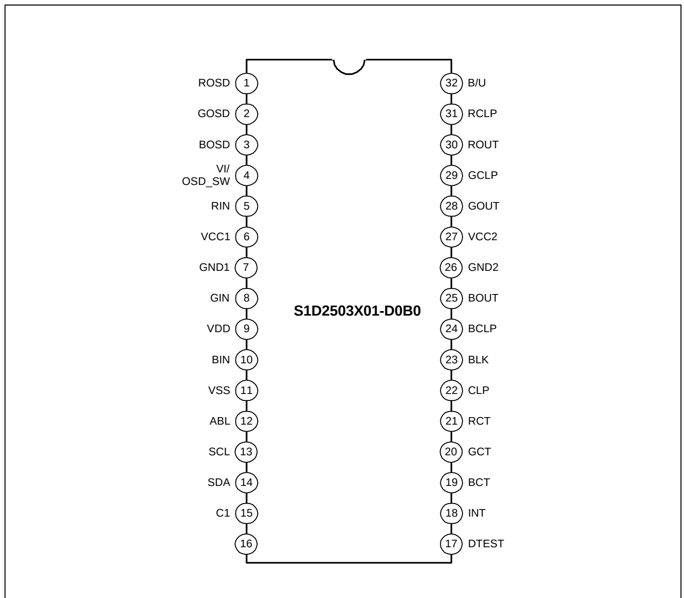
Figure 2. Pin Configuration
