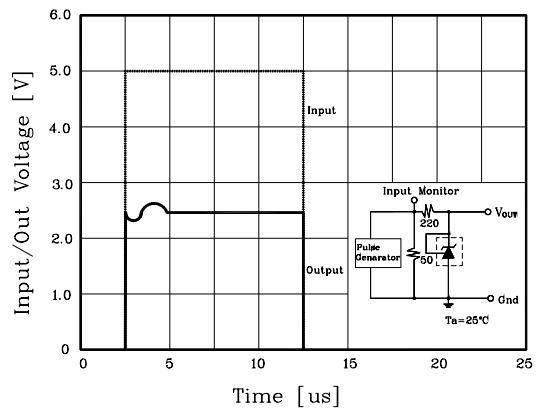
Fig. 9 Pulse response
