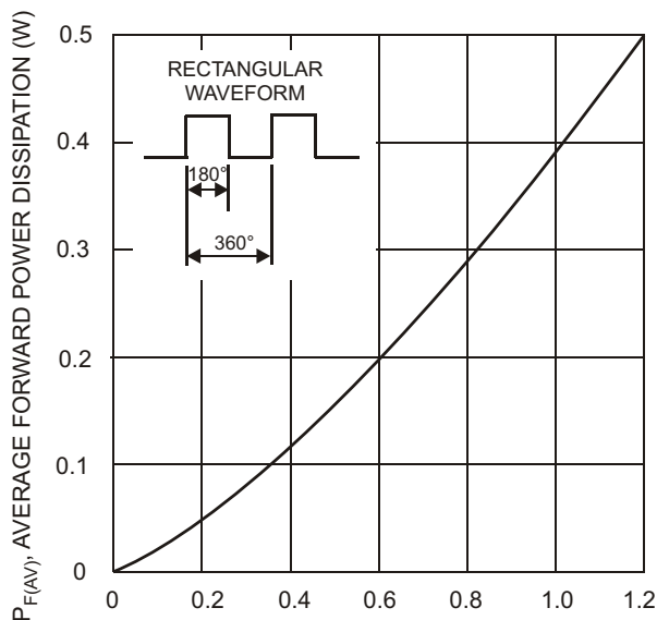
P_{F(AVE)} , AVERAGE FORWARD POWER DISSIPATION (W) I_{F(AVE)} , AVERAGE FORWARD CURRENT (A) Fig. 5, Forward Power Derating
