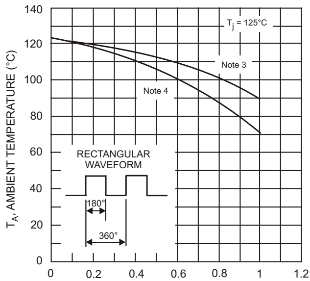
I_{F(AVE)} , AVERAGE FORWARD CURRENT (A) T_A , AMBIENT TEMPERATURE (°C) Fig. 6, Forward Current Derating
