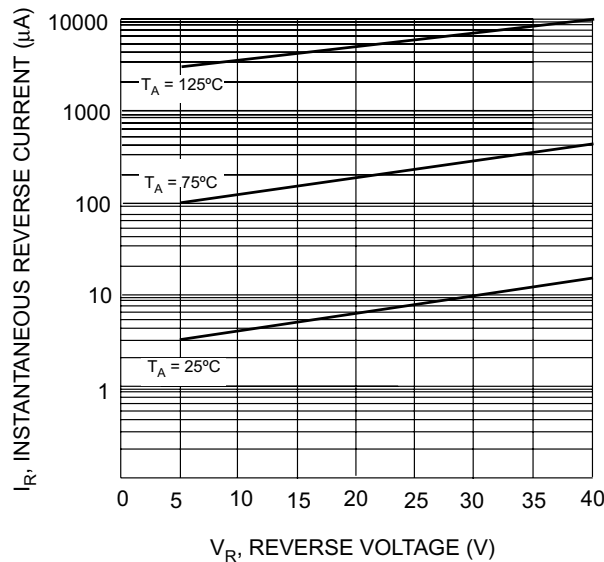
V_R , REVERSE VOLTAGE (V) Fig. 5 Typical Reverse Characteristics
