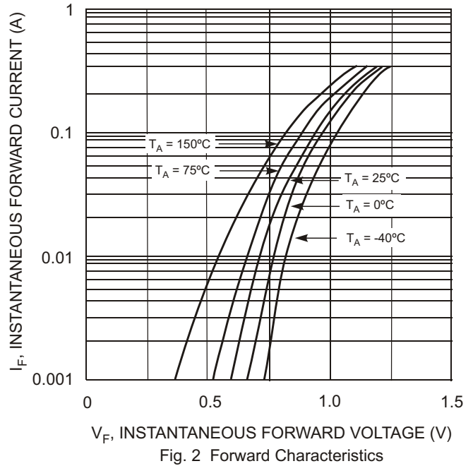
Fig. 2 Forward Characteristics
